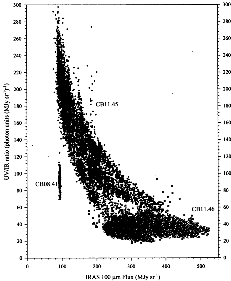
Figure 6. The correlations between the UV flux observed by IUN (photons \text{cm}^{-2} \text{sr}^{-1} \text{s}^{-1} \text{\AA}^{-1} ) and the IRAS 100 \mu\text{m} flux \text{MJy sr}^{-1} ) in plotted for the three DCEs observed. In CB08-41 there is not much variation in either the IR or the UV fluxes; in CB11-45 the UV flux is almost constant while the infrared varies over a factor of 4; and in CB11-46 both vary while keeping the ratio constant.
