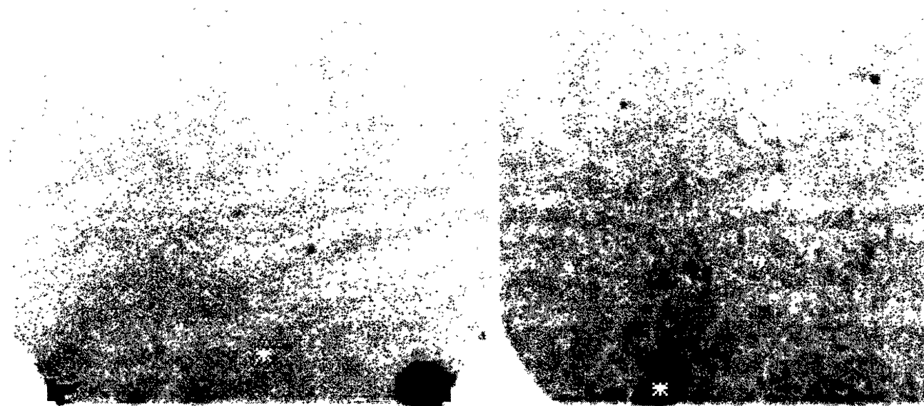
Figure 5. Images from CB11-46 are shown (North to the right and East to the top) for IUN Filter 4 (on the left) and IUN Filter 3. The asterisk is at the same coordinates in both images (RA:05 39 29.26 , Dec:-05 41 25.2). A bright patch is visible in both images and is probably an extended halo to the complex of molecular clouds identified by Ogura & Sugitani (1998) about 15' to the west (bottom) of the image.
