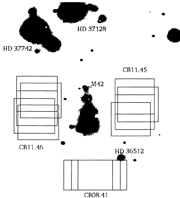
Figure 1. The positions of the 3 Orion Data Collection Events (DCES) are shown on an IUW ( 13^{\circ}1 \times 10^{\circ}3 ) image (with North at the top), with a few of the brighter stars identified: HD 37742 ( \zeta Ori) and HD 37128 ( \epsilon Ori) form part of the Orion belt. There were several pointings within each DCE, with various filters; the IUN field in each pointing is shown by a small box ( 1^{\circ}5 \times 1^{\circ}2 ). The SPIMs scanned over essentially the same field as the narrow field imagers, but with much less sensitivity. Not all of the instruments and pointings provided useful scientific data (for our purposes), for instance the IUW image shown was taken at too low a gain to allow us to detect the diffuse background.
