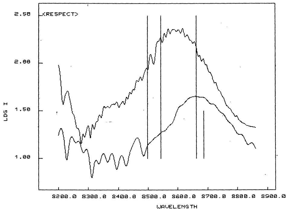
Figure 7. The region around Ca II \lambda 8600 and N I \lambda 8680 on 1987 March 8 (top) and March 30 (bottom). The longer vertical bars are at Ca II \lambda 8498, 8542, 8662, whereas the shorter one is at N I \lambda 8680.
