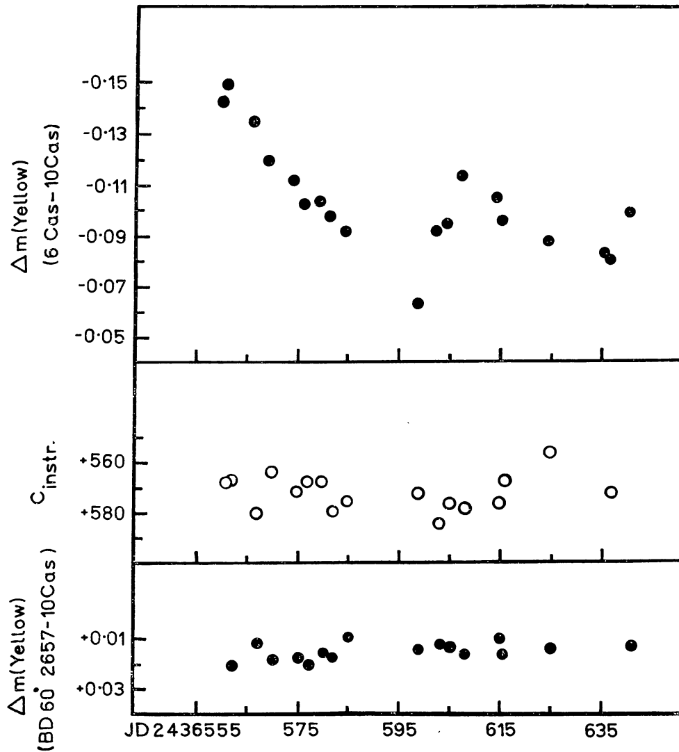
FIG 1 Light and colour variation of 6 Cassiopeiae
