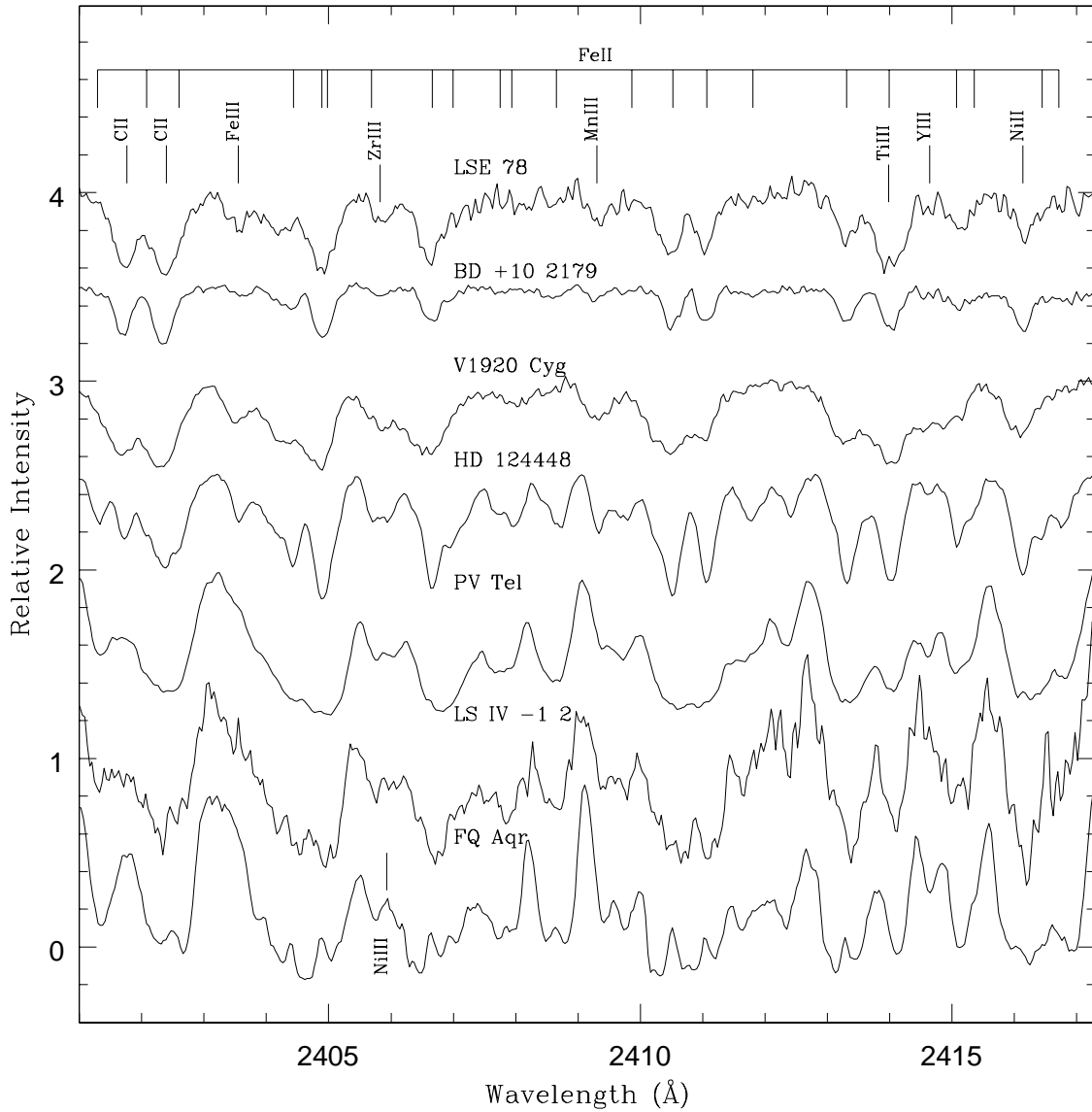
Fig. 2.— A sample of the STIS spectra of the seven EHe stars. The spectra are normalized to the continuum and are shown with offsets of about 0.5 between each. Several lines are identified in this window from 2401 Å to 2417 Å. Stars are arranged from top to bottom in order of decreasing effective temperature.
