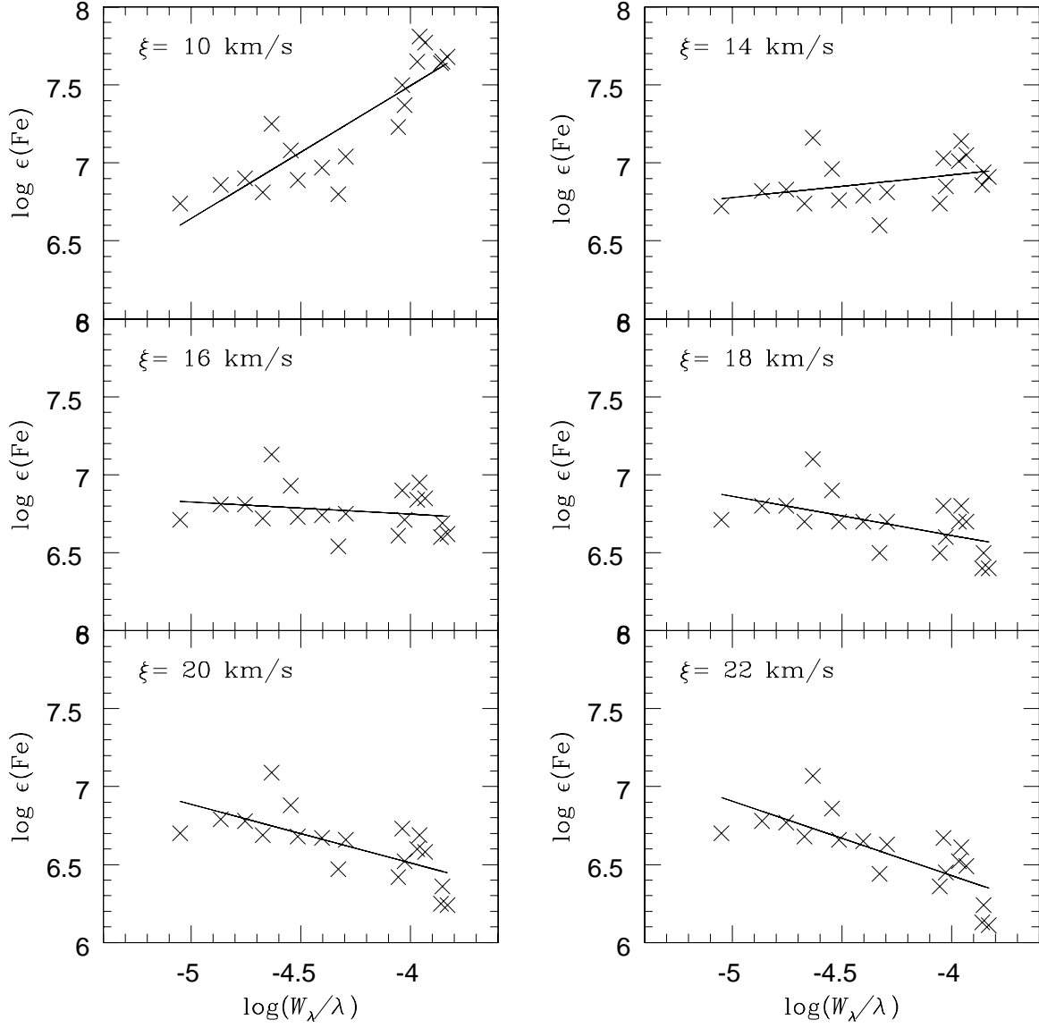
Fig. 3.— Abundances from Fe III lines for LSE 78 versus their reduced equivalent widths ( \log W_\lambda/\lambda ). A microturbulent velocity of \xi \simeq 16 \text{ km s}^{-1} is obtained from this figure.
