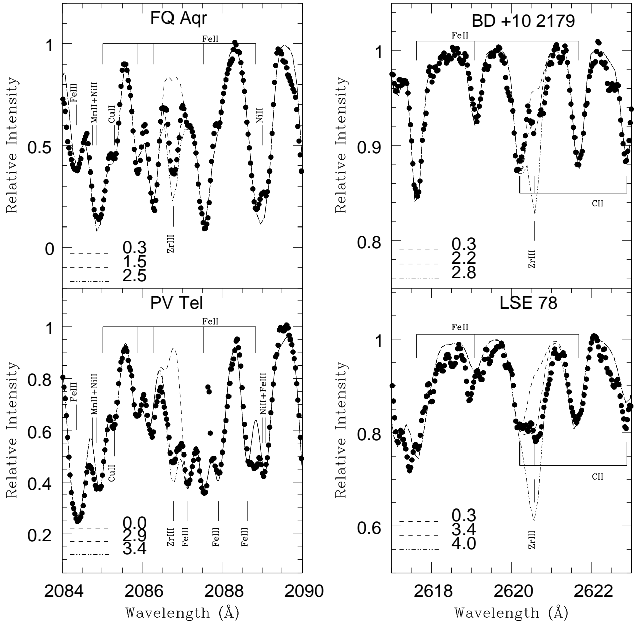
Fig. 15.— The observed spectra of FQ Aqr, PV Tel, BD+10° 2179, and LSE 78 are represented by filled circles. The left-hand panels show the region including the Zr III line at 2086.78Å for FQ, Aqr and PV Tel. The right-hand panels show the region including the Zr III line at 2620.57Å for BD+10° 2179 and LSE 78. Synthetic spectra for three different Zr abundances are shown in each panel for these stars – see keys on the figure. In each panel, the principal lines are identified.
