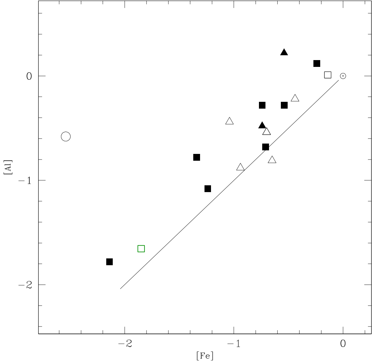
Fig. 12.— [Al] vs [Fe]. Our sample of seven EHes is represented by filled squares. Two cool EHes analysed by Pandey et al. (2001) are represented by filled triangles. The results taken from the literature for the EHes with C/He of about 1% and much lower C/He are represented by open triangles and open squares, respectively. DY Cen is represented by open circle. \odot represents Sun. [Al] = [Fe] is denoted by the solid line.
