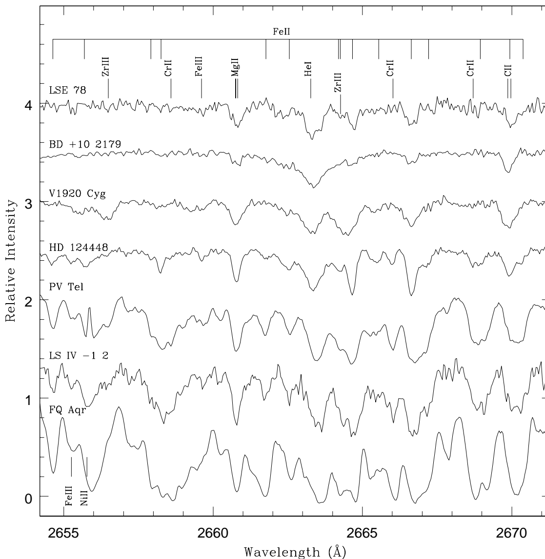
Fig. 1.— A sample of the STIS spectra of the seven EHeS. The spectra are normalized to the continuum and are shown with offsets of about 0.5 between each. Several lines are identified in this window from 2654 Å to 2671 Å. Stars are arranged from top to bottom in order of decreasing effective temperature.
