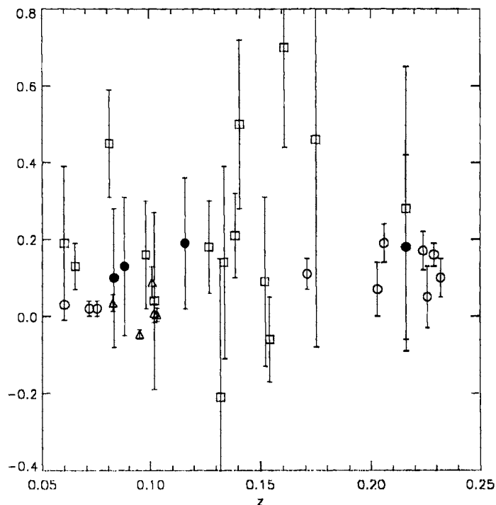
Figure 4.6: The blue fractions in our poor clusters (filled circles), in the poor groups around radio galaxies (squares) studied by Allington-Smith et al. (1993), and in Abell richness 0 clusters (triangles) from the work of Margoniner & de Carvalho (2000). Also shown are f_b values from the pioneering work of Butcher & Oemler (1984) for compact, rich clusters (open circles).
