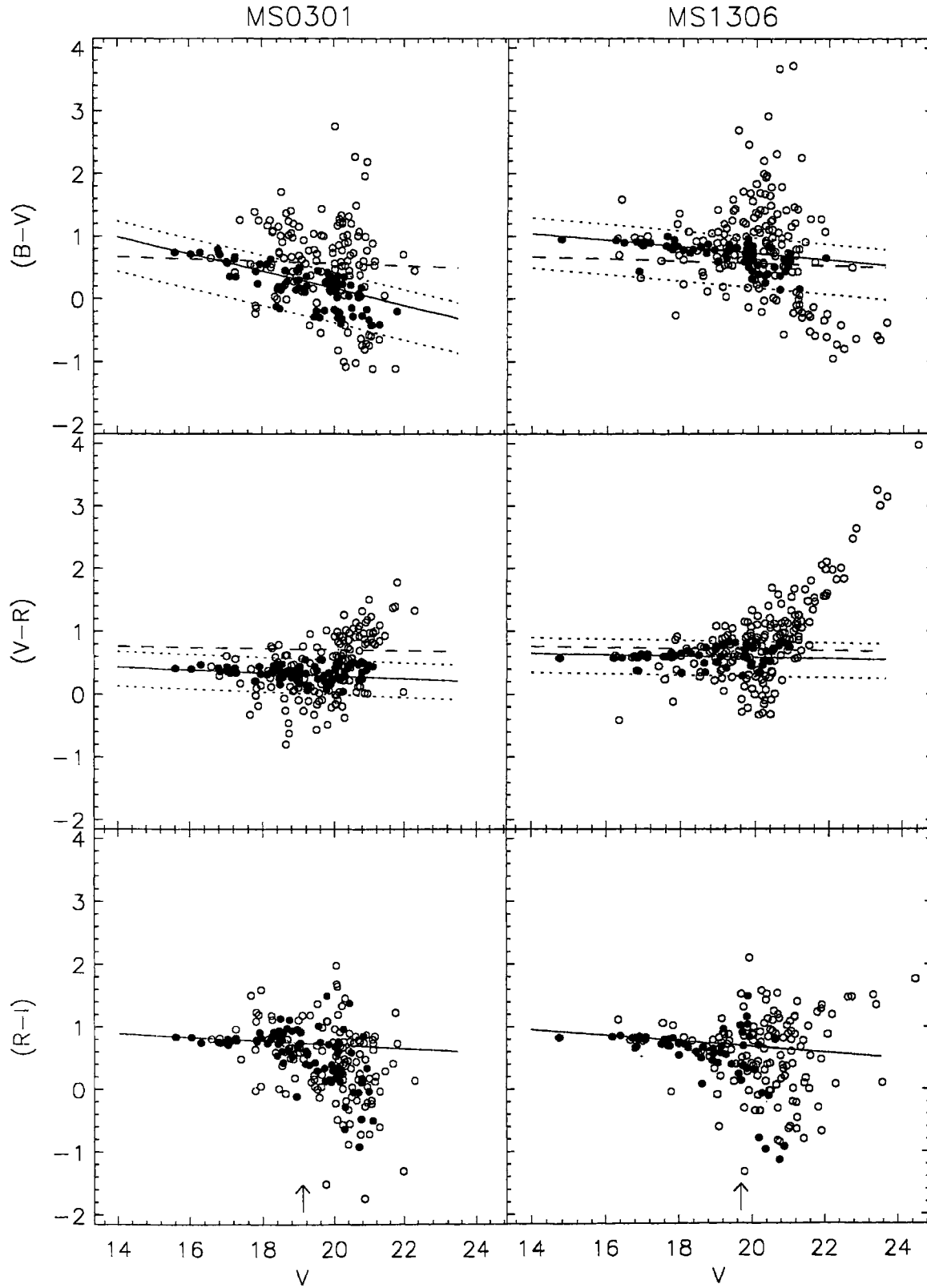
Figure 4.1: Color-magnitude diagrams, (B - V) vs. V , (V - R_C) vs. V , (R_C - I_C) vs. V for galaxies within 0.5 Mpc of the center of MS0301 and MS1306. The solid line in each panel indicates the fit of a linear relation representing the locus of early-type galaxies in the clusters. Filled symbols represent galaxies within the B - V “sequence” in the top panel, and within the V - R “sequence” in the bottom two panels. See text for the definition of “sequence”. The arrows indicate the faintest V magnitude included in the fits. The dotted lines envelop the width of the color-magnitude sequence. The dashed lines represent the CMR expected from the Virgo cluster relation of Visvanathan & Sandage (1977) appropriately redshifted.
