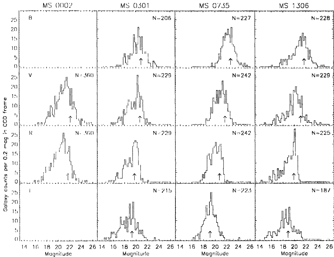
Figure 2.1: Galaxy counts in the CCD frames centered on the BCMs.
