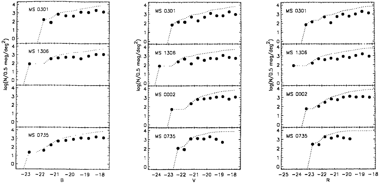
Figure 3.4: Binned luminosity functions of individual poor clusters constructed using cluster sequence galaxies. B , V , R -band LFs are in the left, center and right panels, respectively. The ordinate in each panel is the number of galaxies per 0.5 mag bin within the clustrocentric radii 0.5 Mpc for MS0301 and MS1306 and 0.7 Mpc for MS0002 and MS0735. The abscissa is the absolute magnitude. The solid circles represents the differential LF and the dotted line, the cumulative LF of each cluster including the BCM. Note that we do not estimate the B -band LF for MS0002 due to poor photometric calibration.
