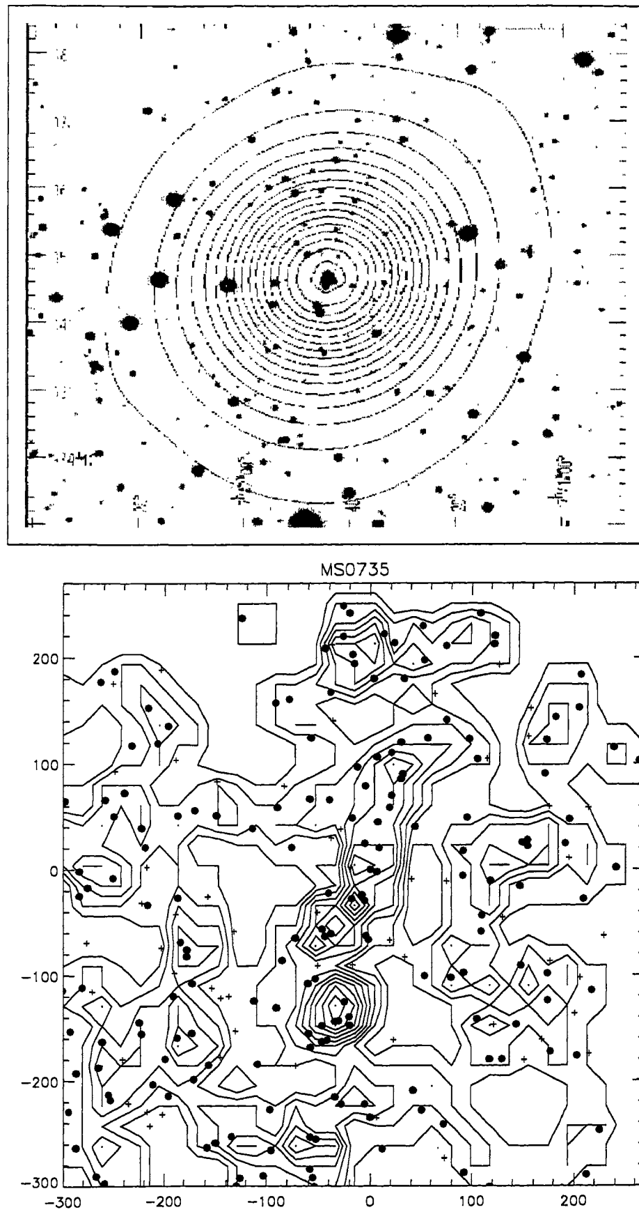
Figure 5.3: Optical and X-ray morphology of MS 0735.6+7421. Axes, gray-scale images and contours as before.
