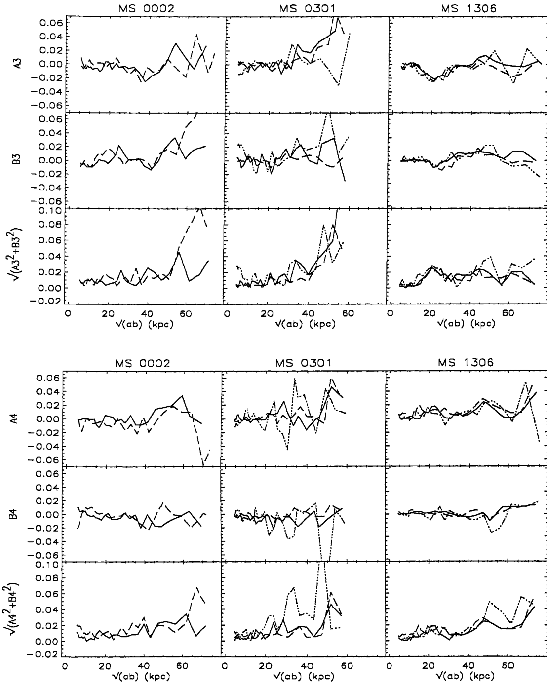
Figure 6.3: Profiles of third- and fourth-order deviations from ellipticity. The abscissa is r = \sqrt{ab} , the geometric mean of the semi-major and semi-minor axis length. Solid line - V, dashed line - R, dash-dotted line - B band.
