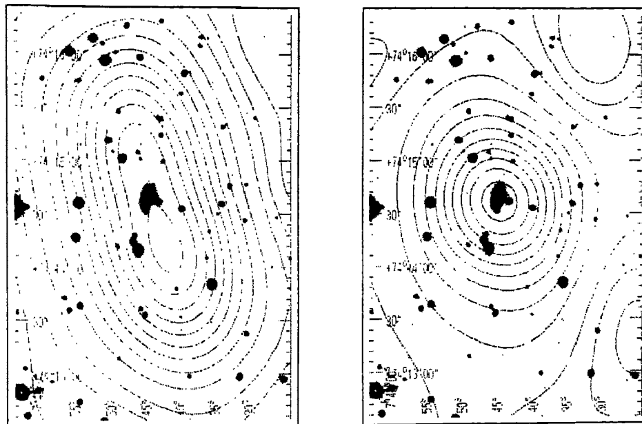
Figure 6.7: The radio maps of 4C +74.13 at 327 MHz (left) and 1.4 GHz overplotted on the optical image.
