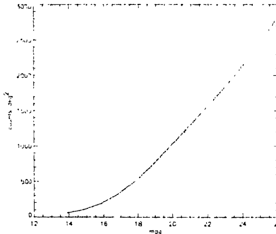
Figure 2.3: Number counts of stars and galaxies in the field of MS1306. The solid line is the prediction of the Bahcall & Soneira (1981) model of Galactic star counts, and the dotted line is the empirical ‘field galaxy’ count of Wilson et al. (1997), both in the V band. Notice that by V \approx 20 mag, galaxies begin to dominate over stars.
