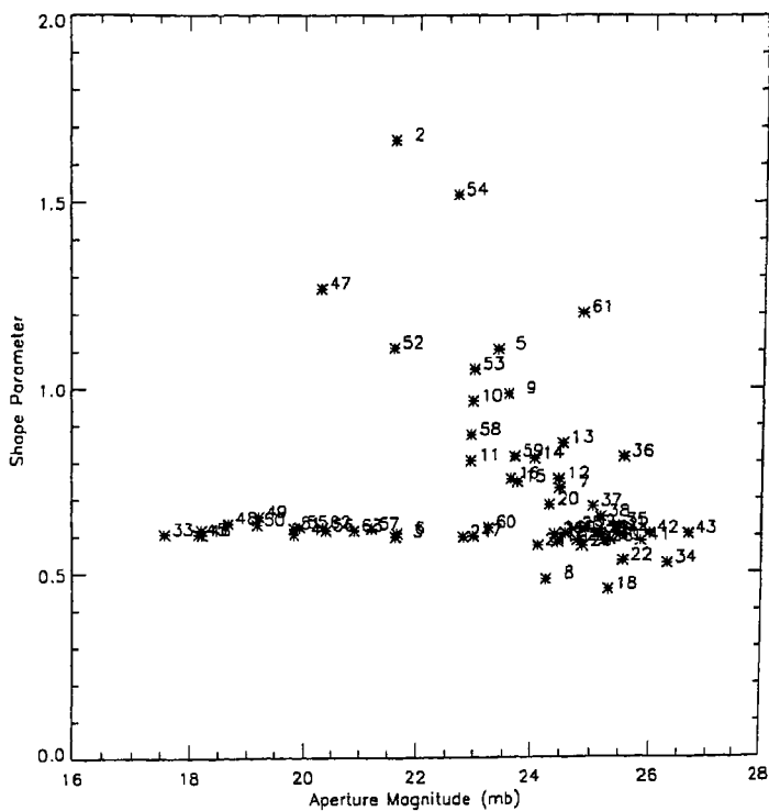
Figure 5.3: GRB 920720: Star-galaxy separation using the shape parameter (see §2.2.5 for details).
