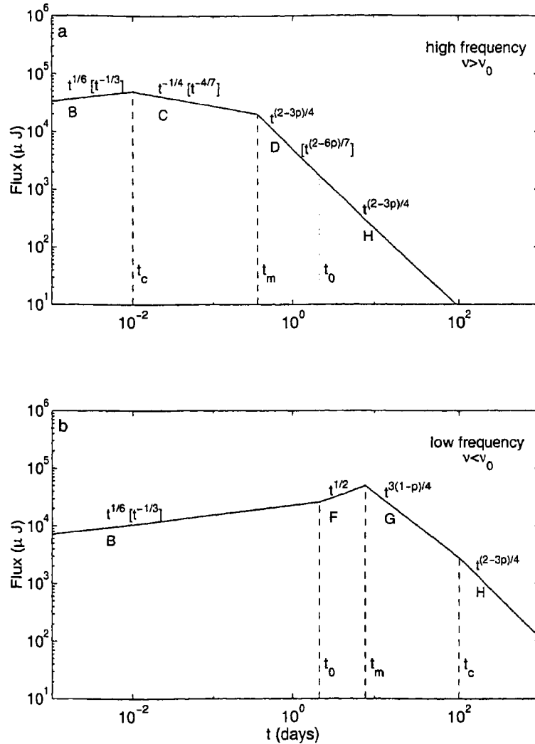
Figure 1.6: Light curve due to synchrotron radiation from a spherical relativistic shock, ignoring the effect of self-absorption. (a) The high frequency case ( \nu > \nu_0 ). The light curve has four segments, separated by the critical times, t_c , t_m , t_0 . The labels, B, C, D, H, indicate the correspondence with spectral segments in Fig. 1.5. The observed flux varies with time as indicated; the scalings within square brackets are for radiative evolution (which is restricted to t < t_0 ) and the other scalings are for adiabatic evolution. (b) The low frequency case ( \nu < \nu_0 ) (Reproduced with kind permission from authors: Sari, Piran & Narayan 1998).
