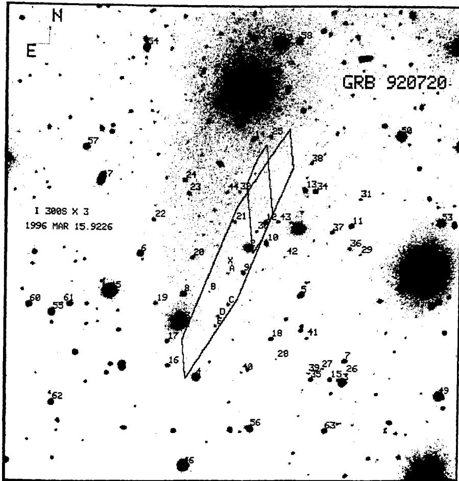
Figure 5.2: GRB 920720: I band image of 300 s \times 3 exposure observed at VBT. The revised ( smaller ) and initial ( larger ) IPN error boxes are shown. The initial center is marked by 'X'. The image scale is 0''.609/\text{pix} and total FOV is 10'.4 \times 10'.4 .
