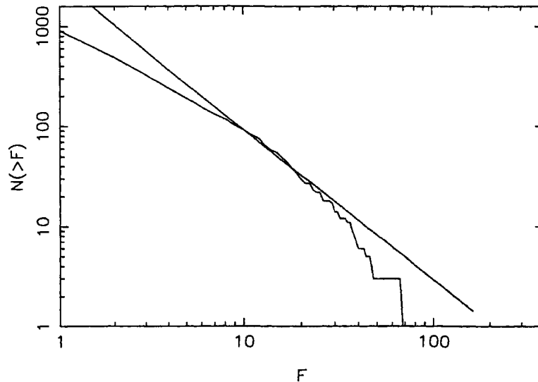
Figure 1.3: \mathcal{N}-F relation for BATSE GRBs.
