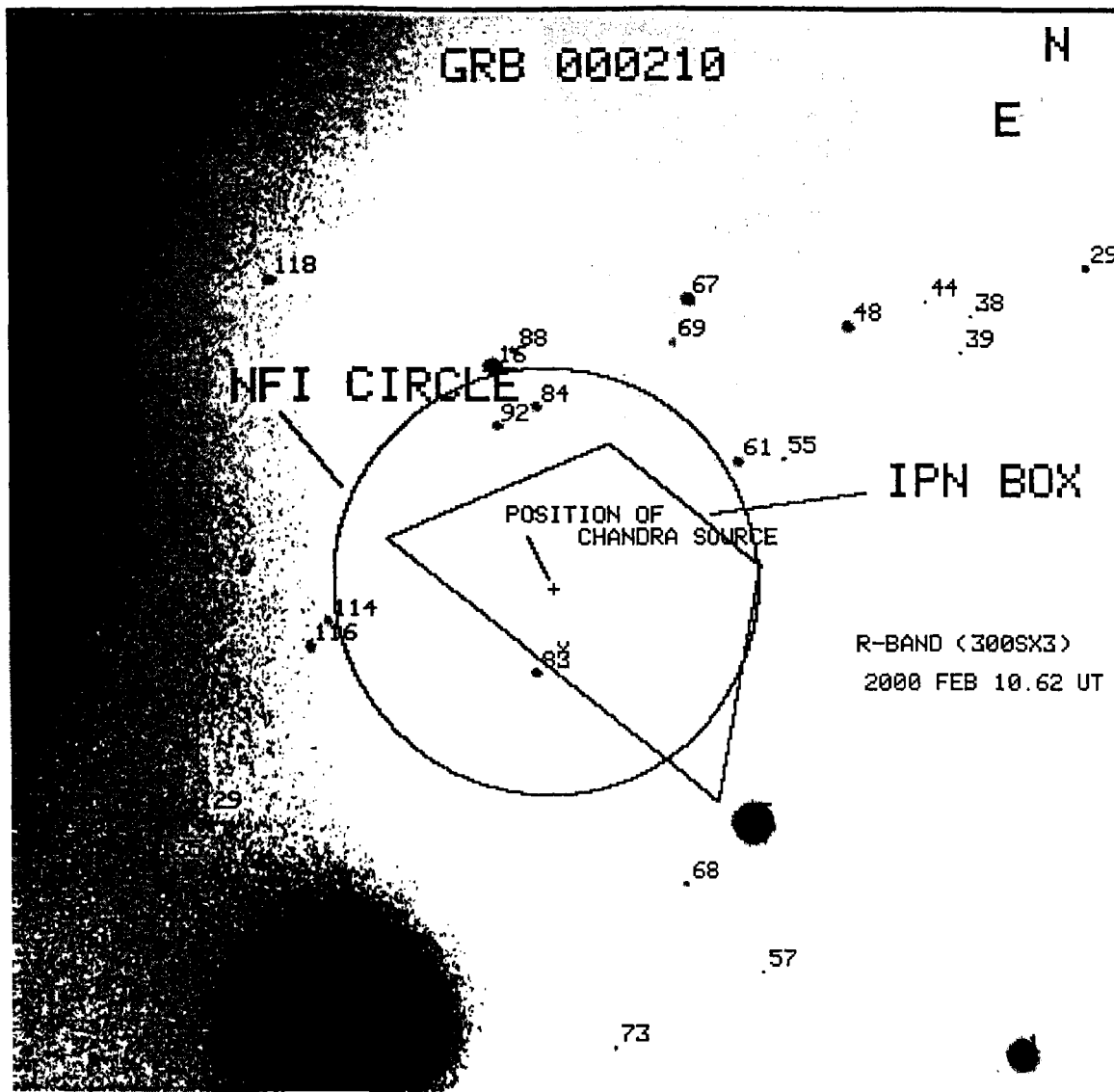
Figure 2.4: The field of GRB 000210 observed at VBT on 10 Feb 2000. In the combined 300s \times 3 image in R-band no source is detected at the position of Chandra source down to the limit R = 18.0 . The NFI error circle as well as the IPN error box are overlaid on the image.
