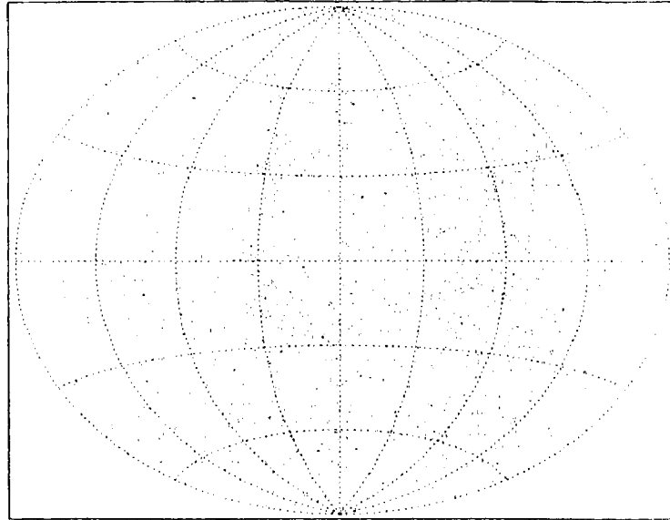
Figure 1.2: Distribution of 2704 BATSE GRBs on the sky.
