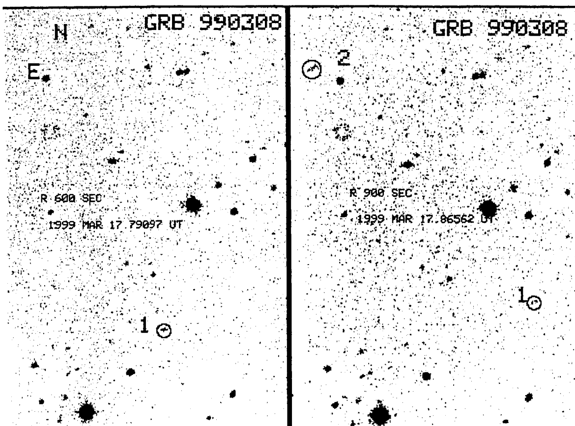
Figure 2.9: Field of GRB 990308 showing two new asteroids : The R-band image of 600 s ( left-panel ) observed at 18.9833 UT and R-band image of 900 s ( right-panel ) observed at 20.775 UT on 17 Mar 1999. The motion of Asteroid-1 can be clearly seen with respect to the background stars. Asteroid-2 was detected in the last two images including the one in the right-panel . Both the asteroids were heading in NW direction with a typical speed of main belt asteroids.
