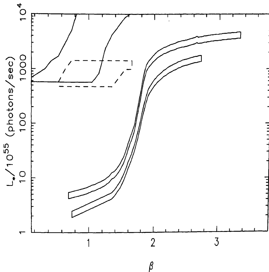
Figure 4.3: The results for the scale-free luminosity function are shown. In this model L_{\min} = 3 \times 10^{-2}L_* and L_{\max} = 100L_* . The regions at the top left of the figure represent the allowed region of likelihood function (i.e. \mathcal{L} > 10^{-4} of maximum likelihood) in L_0 - \sigma plane for afterglow observations. The region with dotted lines corresponds to a run where beaming corrections are applied. The thin regions represent the region of K-S probability P_{\text{ks}} > 0.01 for the consistency between observed and theoretical number count-flux relation. These correspond, with increasing photon luminosity, to GRB evolution models III and IV discussed in the text. The allowed regions for models I and II fall below the allowed regions for the models shown.
