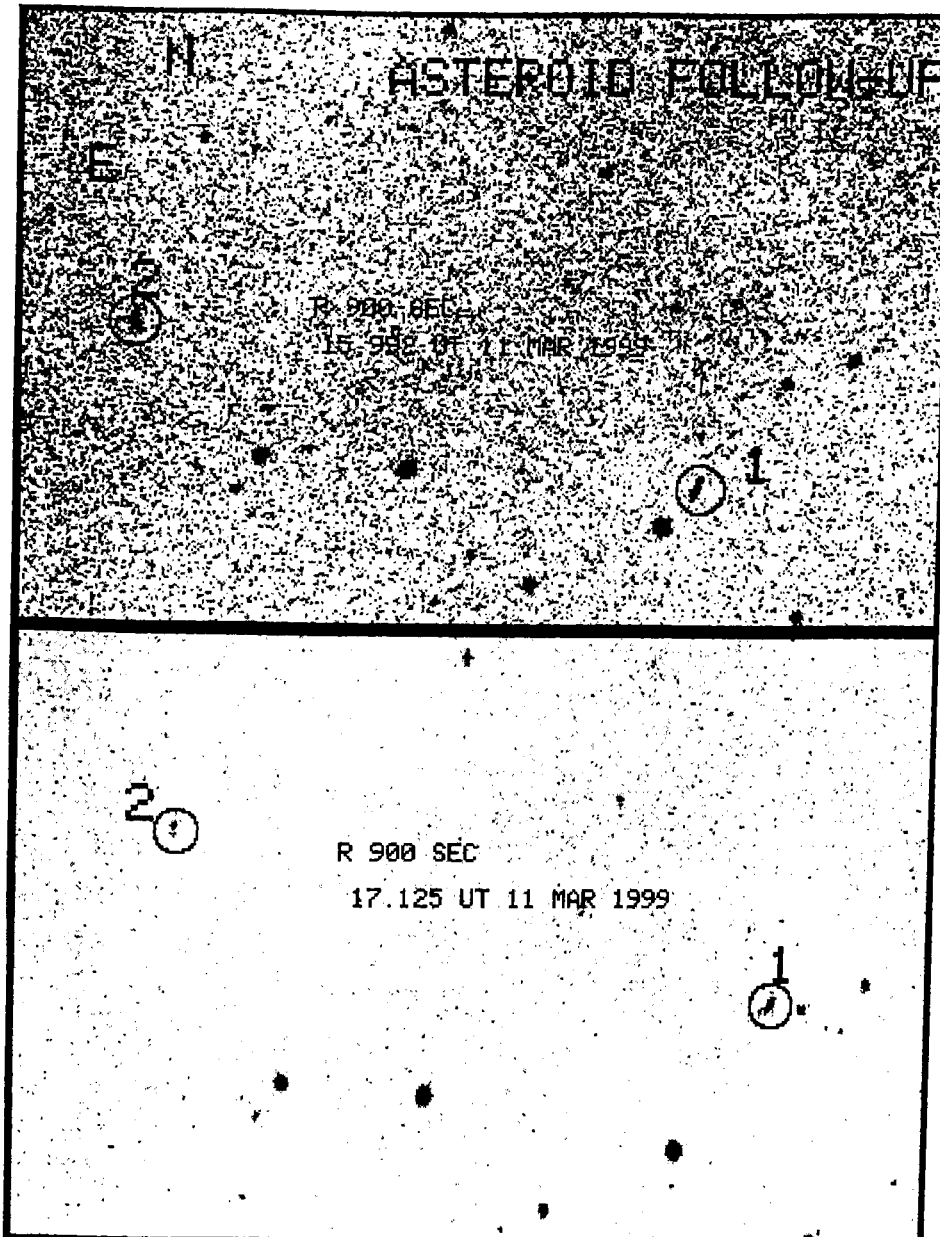
Figure 2.10: Follow-up of Asteroids: Region of the sky with predicted positions of asteroids was observed on 11 Mar 1999. In a series of 5 images both the asteroids were recovered. Asteroid motion in NW direction can be clearly seen with respect to the background stars in above images.
