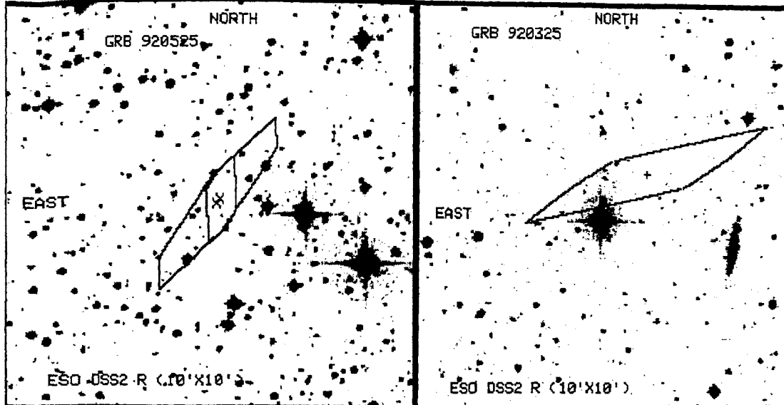
Figure 5.1: DSS2 R-band images : left-panel : The field of GRB 920525; The revised (central) and initial (outer) rectangles are drawn using the co-ordinates of the corners of IPN 3 error box from Laros et al. (1998) and Vrba (e-mail communication) respectively. right-panel : The field of GRB 920325 with IPN 3 error box drawn from Laros et al. (1998).
