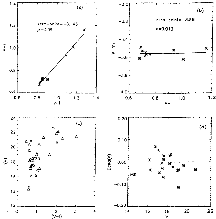
Figure 5.9: GRB 920525: (a) & (b) show the calibration solutions, (c) the color-magnitude diagram and (d) the residual (computed - standard) V magnitude plotted v/s standard V magnitude. (V-I) , V and f(V-I) , fV represent standard (from Vrba et al. ) and computed color and magnitudes, respectively.
