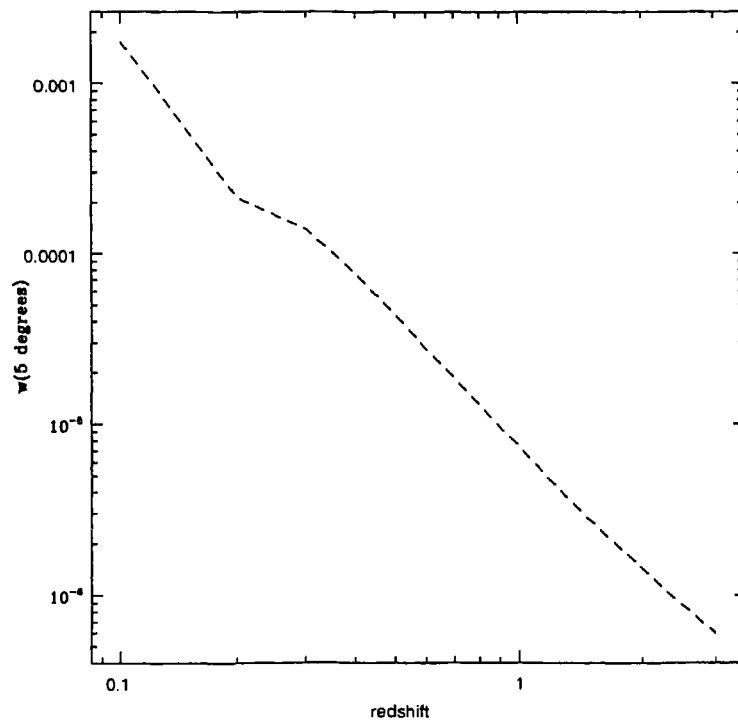
Figure 6.2: Theoretical two-point angular correlation function using the predictions for the \Lambda CDM model is shown as a function of depth (redshift) of the sample. The quantity plotted is the absolute value of the two-point correlation function at \theta = 5^\circ .
