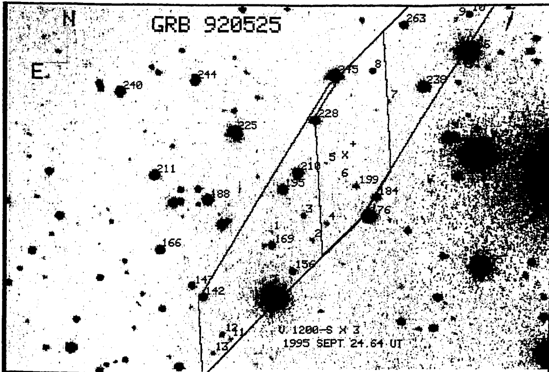
Figure 5.8: GRB 920525: The CCD image in V-band of 20 min \times 3 exposure taken with Astromed CCD 578 \times 385 at VBT. The FOV is \sim 5'.3 \times 3'.5. The revised (inner) and initial (outer) error boxes are drawn using the box co-ordinates from Laros et al. (1998) and Vrba (2000; e-mail communication) respectively. The object marked as #225 is a bright galaxy \sim 30'' from the box center.
