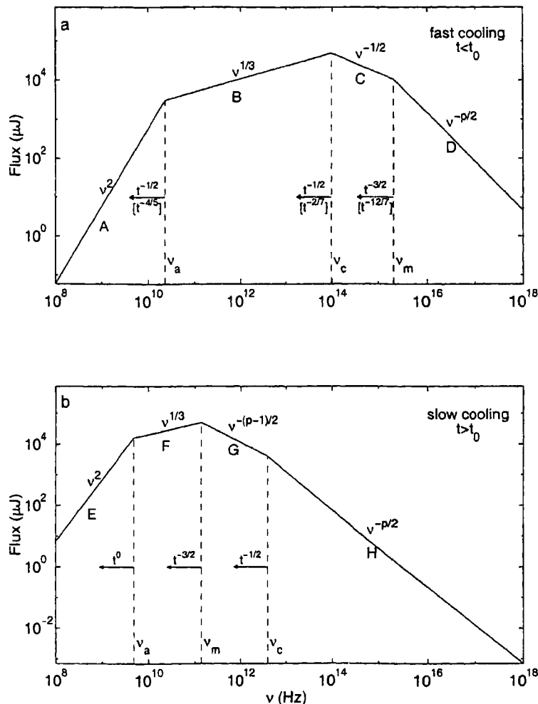
Figure 1.5: Synchrotron spectrum of a relativistic shock with a power-law distribution of electrons. (a) The case of fast cooling, which is expected at early times ( t < t_0 ) in a \gamma -ray burst afterglow. The spectrum consists of four segments, identified as A, B, C, D. Self-absorption is important below \nu_a . The frequencies, \nu_m , \nu_c , \nu_a , decrease with time as indicated; the scalings above the arrows correspond to an adiabatic evolution, and the scalings below, in square brackets, to a fully radiative evolution. (b) The case of slow cooling, which is expected at late times ( t > t_0 ). The evolution is always adiabatic. The four segments are identified as E, F, G, H (Reproduced with kind permission from authors: Sari, Piran & Narayan 1998).
