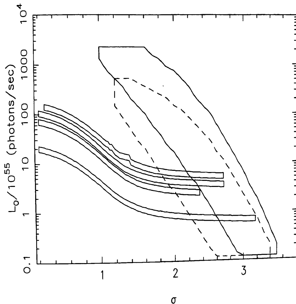
Figure 4.1: The results for the Log-normal luminosity function are shown: The bigger regions in the center enclose the allowed region of likelihood function (i.e. \mathcal{L} > 10^{-4} of maximum likelihood) in L_0 - \sigma plane for afterglow observations. The region with dotted lines corresponds to a run where beaming corrections are applied. The 4 contours on the left side represent the region of K-S probability P_{ks} > 0.01 for the consistency between observed and theoretical number count-flux relation. They correspond, from bottom to top (with increasing luminosity) to four models 1-4 respectively of GRB evolution described in the text.
