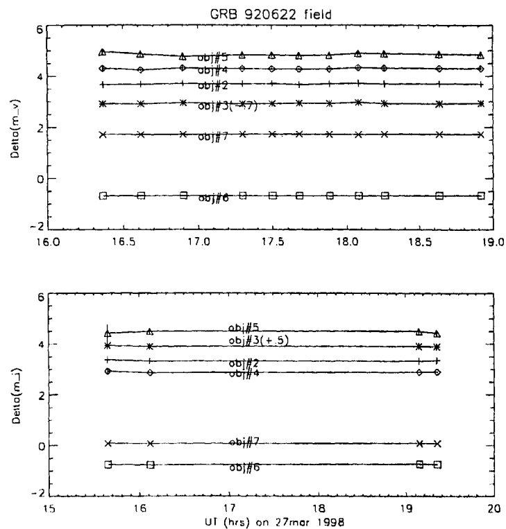
Figure 2.8: Monitoring of objects in GRB 920622 field: On the y-axis differential instrumental magnitude of 6 objects with respect to a GSC star in the field is plotted as a function of time.
