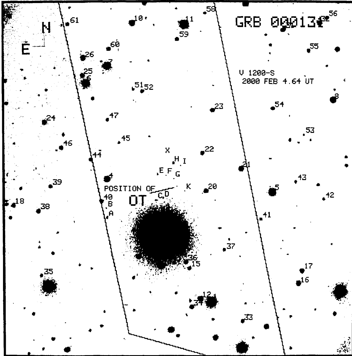
Figure 2.3: GRB 000131 observed in V-band (20 min) using 2.34 m VBT on 2000 Feb 4.64 UT. The IPN error box is overlaid on the \sim 10'.4 \times 10'.4 FOV of VBT. The position of the possible afterglow (Pedersen et al. 2000) is marked on the image.
