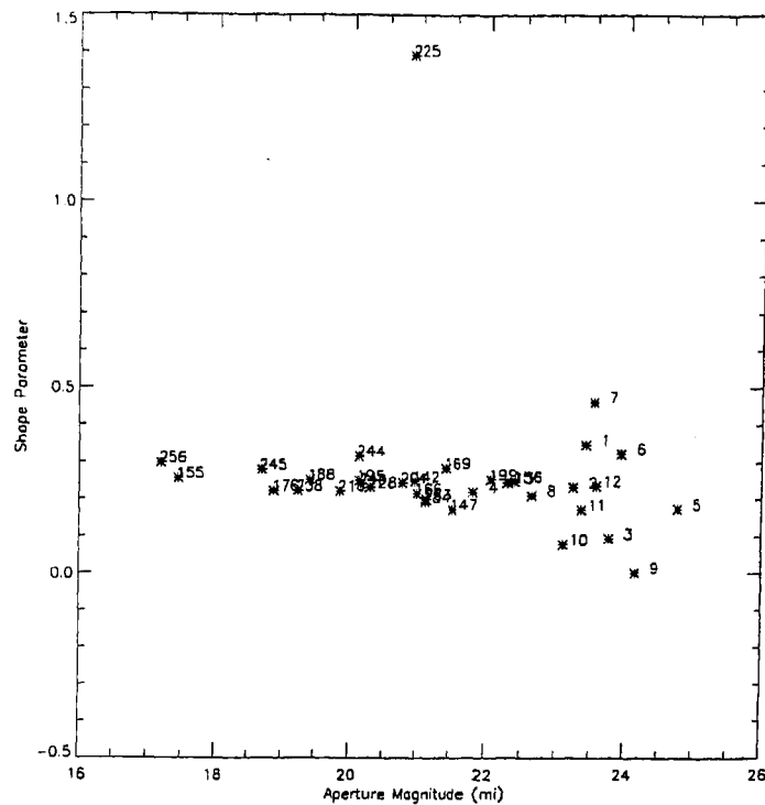
Figure 5.10: GRB 920325: Star-galaxy separation using the shape parameter (see §2.2.5 for details).
