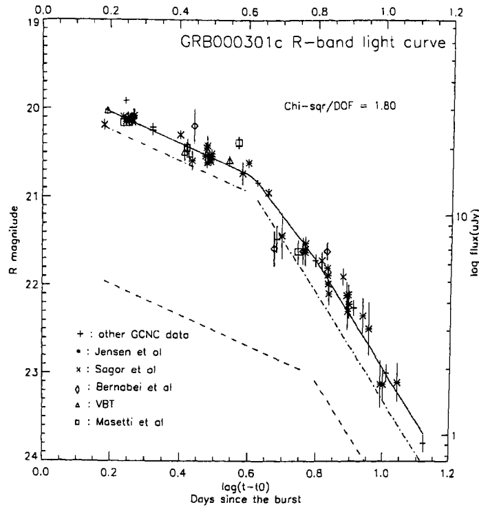
Figure 3.3: GRB000301c R-band light curve: The dotted and dashed lines represent the major and minor burst which add up to give the light curve shown as a solid line.
