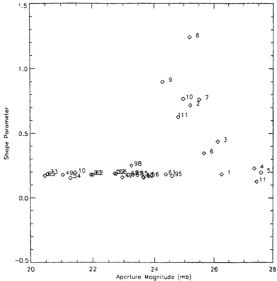
Figure 2.2: Star-Galaxy separation: The figure shows a plot of aperture magnitude v/s a shape parameter (see text for details). The horizontal sequence of objects are stellar in origin. The objects numbered 2, 3, 6-10 are identified as galaxies.
