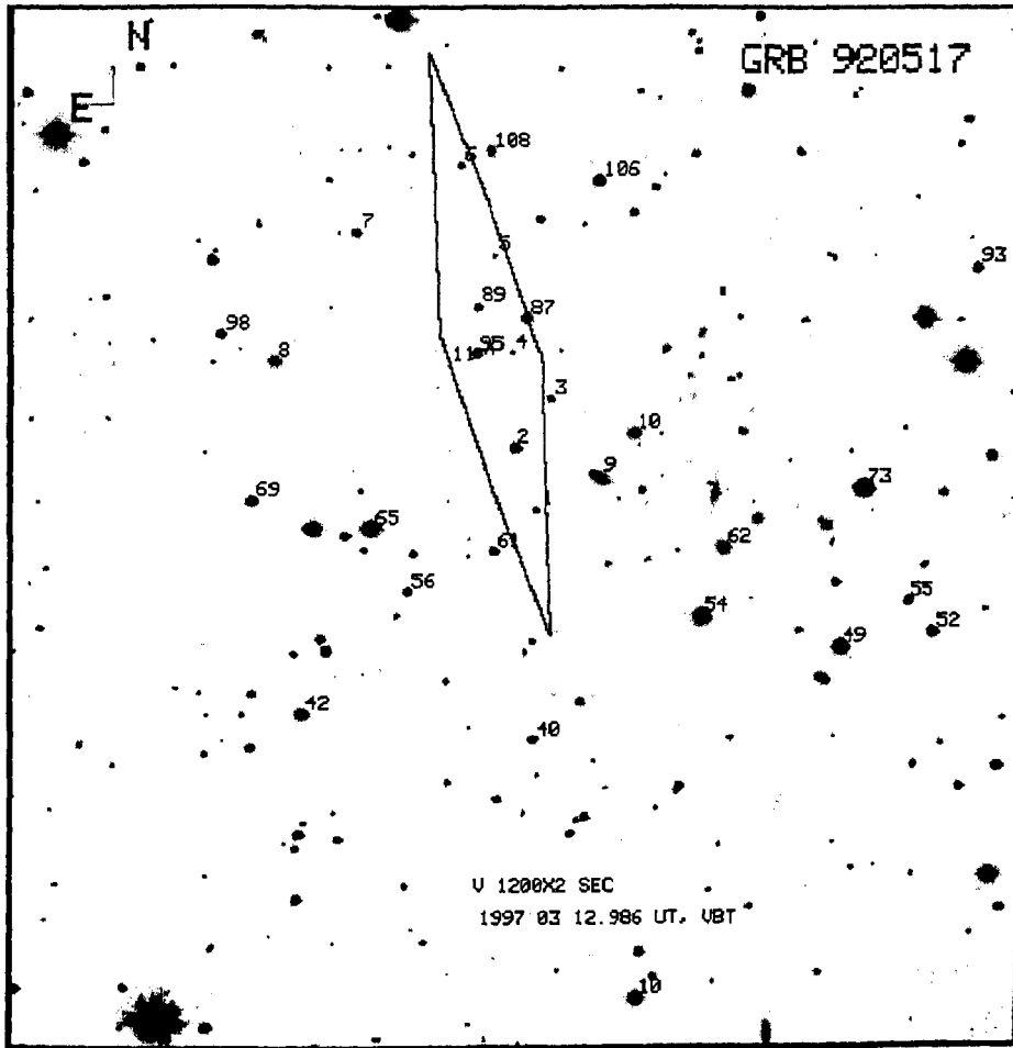
Figure 5.5: GRB 920517: V-band image observed with VBT. The objects marked outside the error box are local standards chosen from the field photometry provided by Henden (2001) and are used to calibrate the objects inside the error box. The total FOV is 10'.4 \times 10'.4 .
