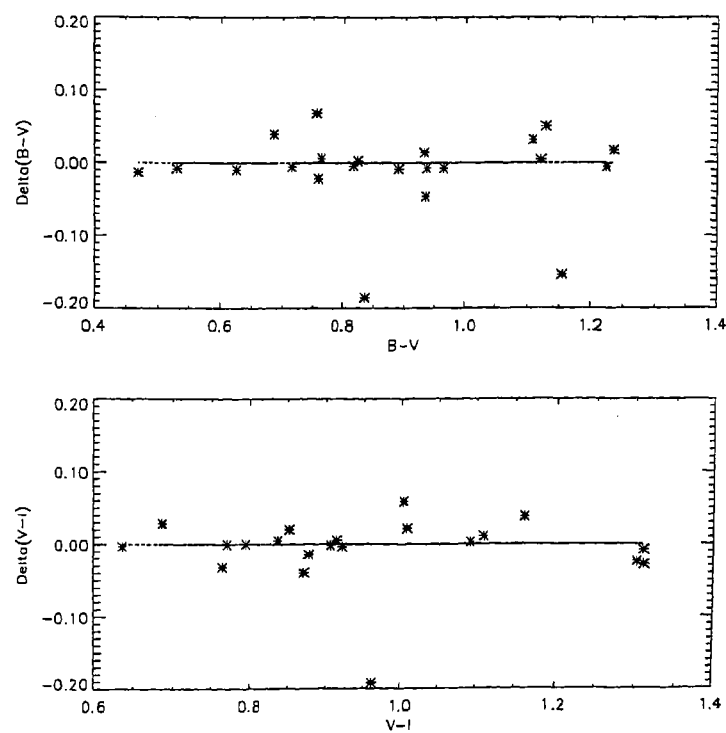
Figure 5.6: GRB 920517: The residual (computed – standard) colors B–V ( upper panel ) and V–I ( lower panel ) are plotted against the respective standard colors.
