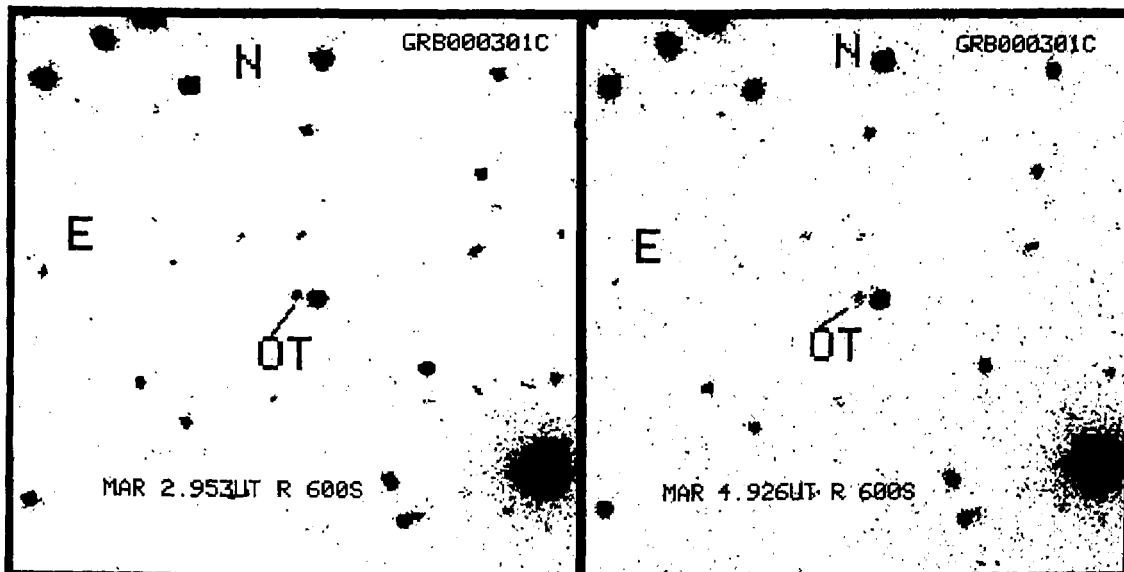
Figure 3.1: The R-band images of GRB000301c field of exposure 600 s each taken on Mar 2.9953UT and Mar 4.9257UT where the fading of OT is clearly seen. The image portions shown here are of size 2'.6 \times 2'.6 ; North is up and East is to the left.
