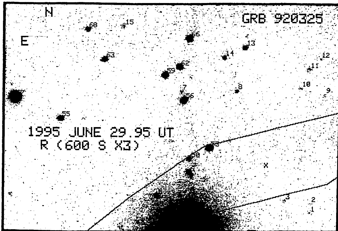
Figure 5.11: GRB 920325: The combined R-band image of 600 \times 3 sec exposure observed with VBT on 29 June 1995. The FOV is \sim 5'.3 \times 3'.5 . The revised IPN 3 error box (Laros et al. 1998) is shown.
