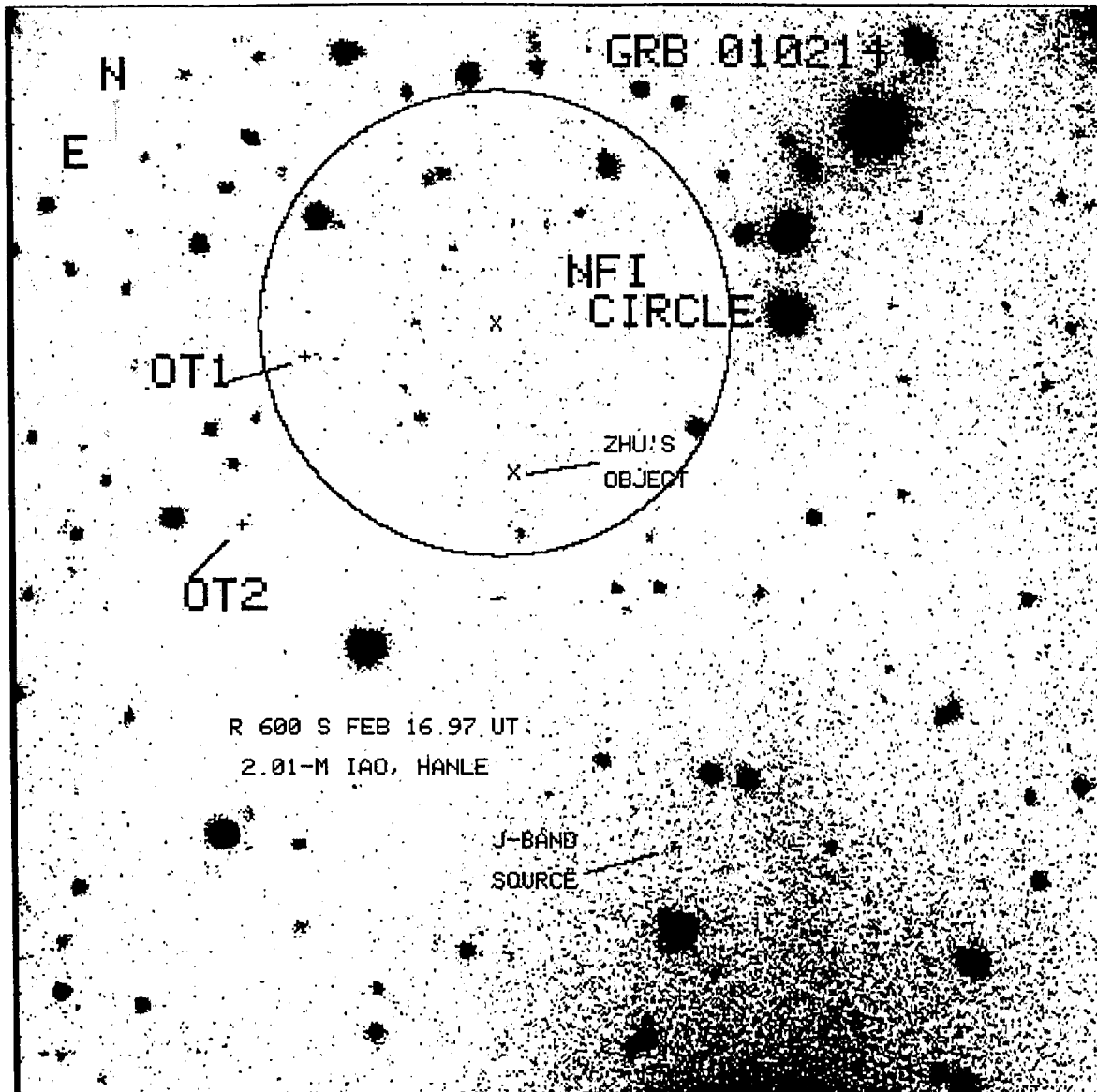
Figure 2.5: The first GRB follow-up from the new 2.01 m telescope at IAO, Hanle: CCD image of the field of GRB 010214 observed on 16 Feb 2001 in R-band. FOV is \sim 4'.7 \times 4'.7 ; The image scale is 0''.274/\text{pix} . The NFI error circle is shown; OT1 and OT2 are positions of optical afterglow candidates reported by Rol et al. (2001a). The position of possible afterglow candidate reported by Zhu et al. (2001) and the J-band source (Di Paola et al. 2001a) are also shown. The faint objects inside the NFI error circle are below the DSS limit.
