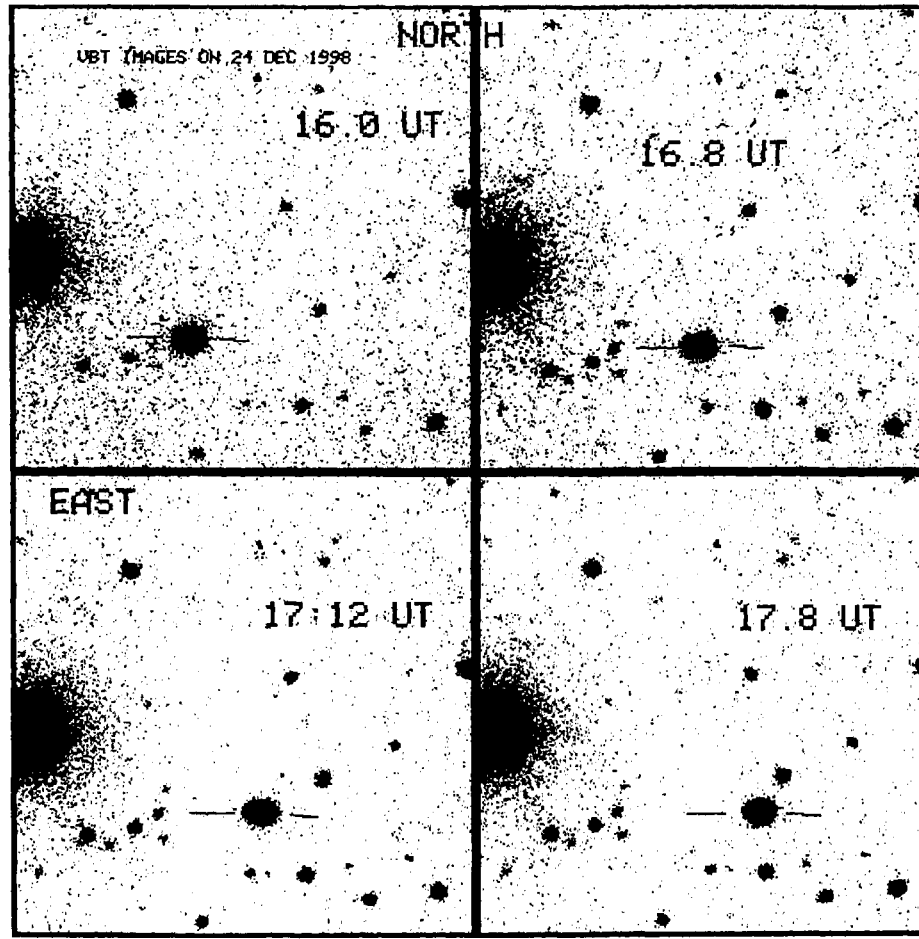
Figure 2.11: FOV of GRB 981220: Figure shows the motion of asteroid '1618 dawn' towards South-West direction with respect to the background stars in 4 successive CCD frames. North is top and East is to the left. Each frame is of size 2'.5 \times 2'.5 .
