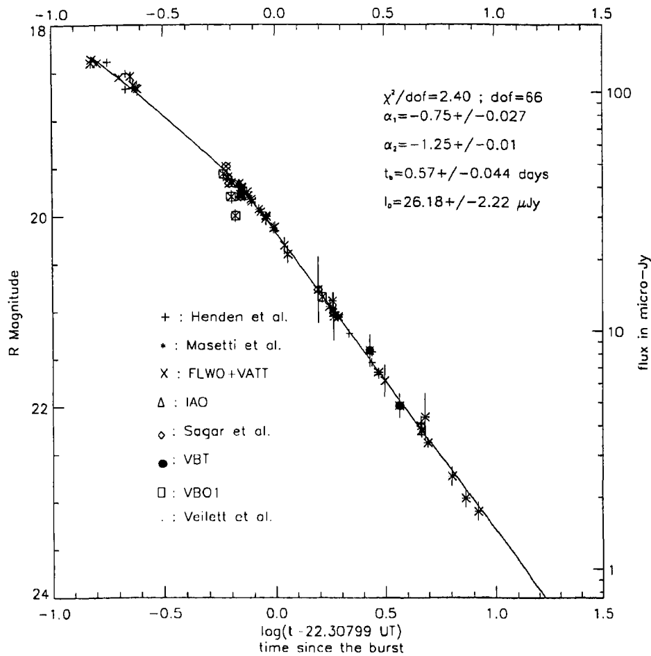
Figure 2.7: GRB 010222: R-band light curve of the afterglow.
