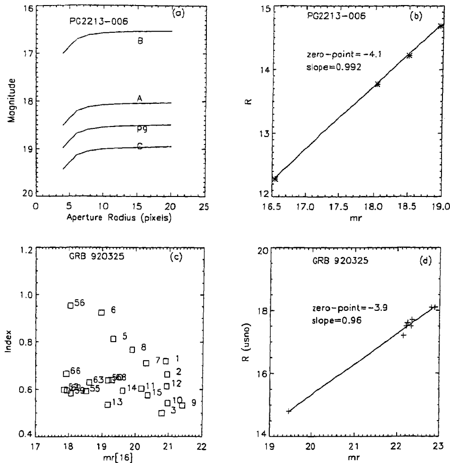
Figure 5.12: GRB 920325: Growth curve (a) and calibration plot (b) using the nightly standard star observation; star-galaxy separation using the shape parameter (see §2.2.5 for details) (c). The instrumental v/s R magnitude (USNO-A2.0) is also shown in (d).
