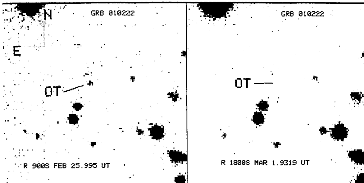
Figure 2.6: The fading behaviour of afterglow of GRB 010222 can be seen in the CCD images observed from 2.34 m VBT. The OT detected on 25th Feb 2001 ( left-panel ) has disappeared in the image taken on 1st Mar, 2001 ( right-panel ). The FOV here is 1'.3 \times 1'.3 .
