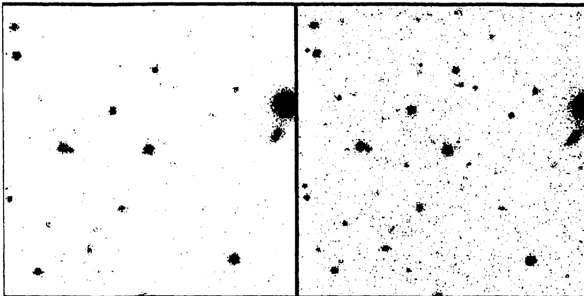
Figure 2.1: R-band (600 s) images of the same field taken under different seeing conditions. The FOV is \sim 3' \times 3' ; the image on the right-panel detects many faint objects as compared to the left-panel image.
