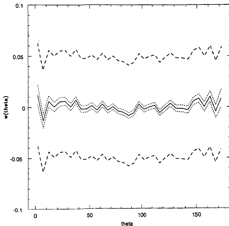
Figure 6.1: The two-point angular correlation function for the BATSE catalog (2494 objects) and the 1\sigma error bars are shown. The solid line corresponds to the two-point correlation function. The dotted lines show the 1\sigma errors given by Eq. (6.4).
