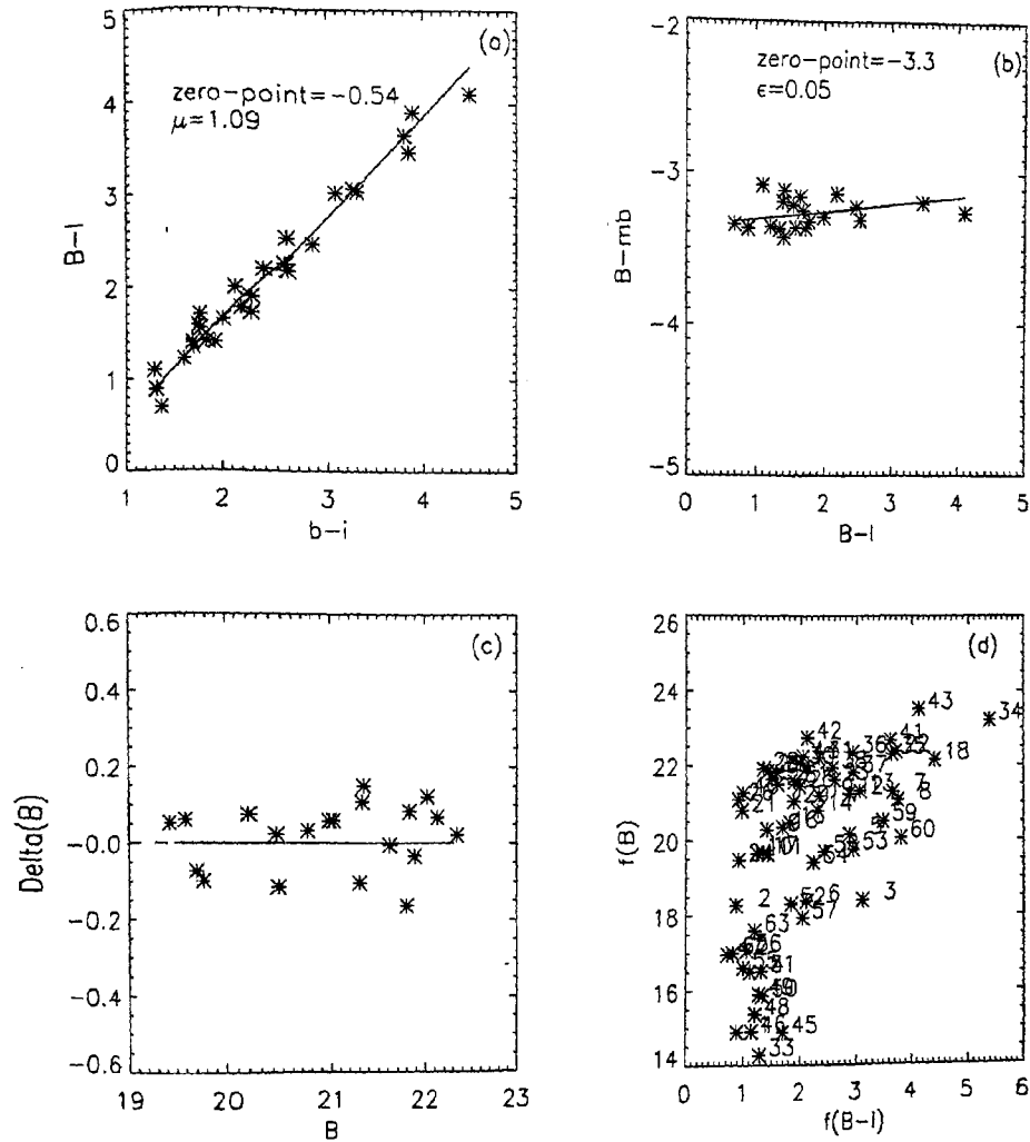
Figure 5.4: GRB 920720: (a)&(b) Calibration solutions (c) residual B (i.e, computed - standard) v/s B (d) color-magnitude diagram. Here, B and (B-I) represent the standard values (taken from Vrba et al. ); fB and f(B-I) represent the computed values.
