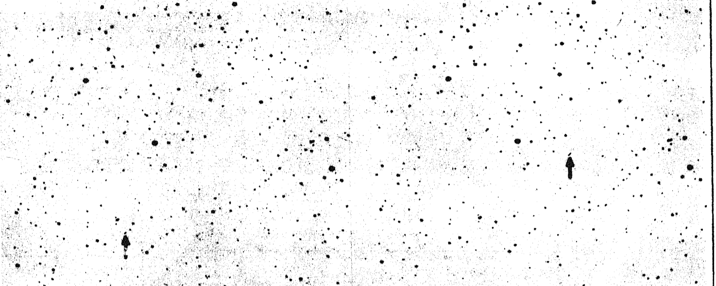
Asteroid number 229 "Adelinda" photographed with the Kavalur Schmidt.
