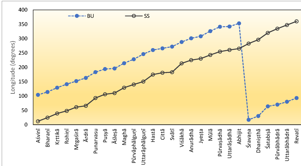
Figure 3: Longitudes of the lagna in BU corresponding to the longitudes of the junction stars ( yogatāra ) from SS. The sudden jump (360+) in the values of BU for the last six points is because of the apparent difference of about 90°.
