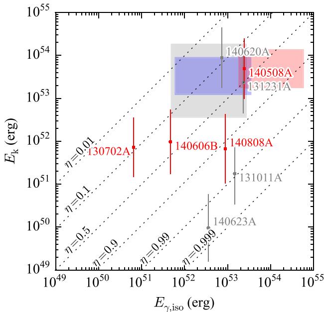
Figure 9. Fireball kinetic energy E_{k,\text{iso}} at t = T_{90} as estimated from X-ray flux vs. rest-frame isotropic-equivalent gamma-ray energy E_{\gamma,\text{iso}} . Red points denote bursts for which E_{k,\text{iso}} can be reliably estimated from the Swift XRT data; gray points denote bursts for which the calculation of E_{k,\text{iso}} may have extreme model dependence. Dashed lines are lines of constant radiative efficiency \eta = E_{\gamma,\text{iso}} / (E_{k,\text{iso}} + E_{\gamma,\text{iso}}) . The gray, blue, and red rectangles show the 1\sigma parameter ranges of Swift BAT, BAT+GBM, and BAT+LAT long GRBs from Racusin et al. (2011).
