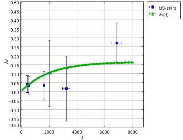
Fig. 1. A_V(d) relation for area 1
