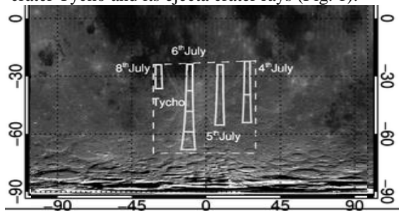
Fig. 1: Distinct elemental measurements were made for these C1XS observed ground-tracks over southern lunar highlands [4,5].
