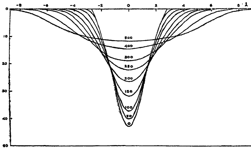
H \alpha 4026 ( \tau Sec) Relatively Broadened Profiles Ordinate is Percentage of Absorption
