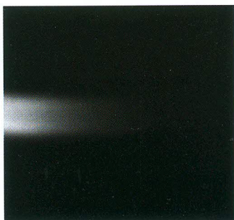
A representative H-alpha image: A slit width of 300 microns at the East limb of the sun was used with an exposure time of 126 ms at 7.1 Hz.
