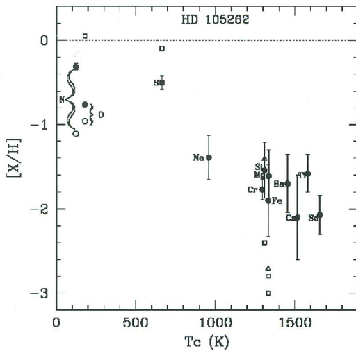
Abundance [X/H] versus condensation temperature for HD 105262 (filled circles). The authors have included the abundance of the hot post-AGB stars HD 137569 (open squares) (Giridhar & Arellano Ferro 2005) and R OA 5701 (empty triangles) (Moehler et al. 1998). Open circles indicate the N and O values after the correction for N LTE.
