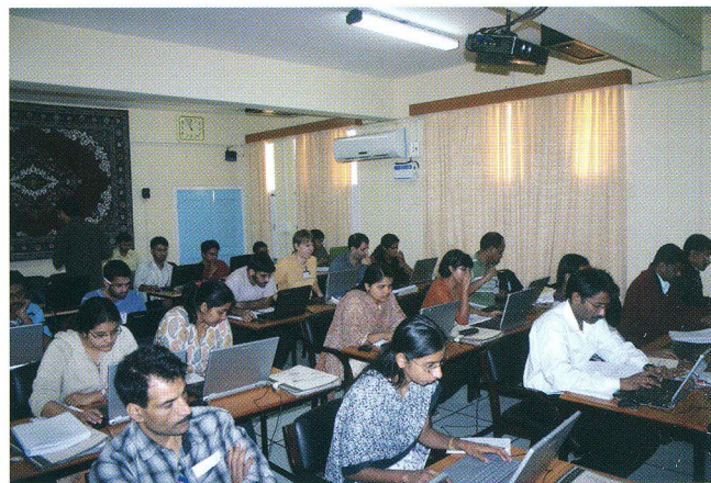
The participants engaged in an astrostatistics tutorial.
