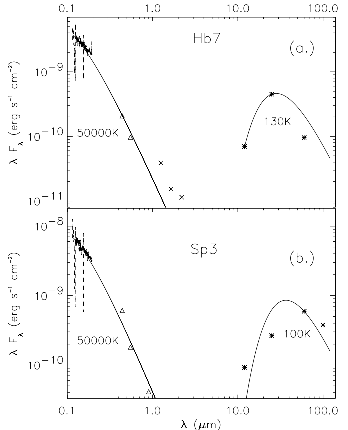
Fig. 2. Energy distribution of Hb7 a) and Sp3 b) from the UV to the far infrared is shown. The data is corrected for interstellar reddening using E(B - V) = 0.19 for Hb7 and E(B - V) = 0.159 for Sp3. IUE data (dashed line) is plotted along with BVI (open triangles), JHK (crosses) and IRAS photometry (asterisk marks).
