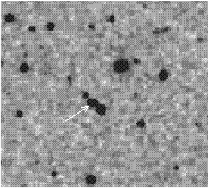
Fig. 3. 2MASS image of Hb7 in K band.
