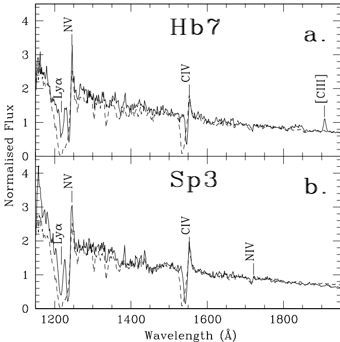
Fig. 1. The dereddened spectra of Hb7 a ), E(B - V) = 0.19 and Sp3 b ), E(B - V) = 0.159 are plotted along with the dereddened SWP spectra of a standard O3-dwarf star (HD 93205, E(B - V) = 0.34 ) from the standard star atlas by Heck et al. (1984). The standard star spectrum is represented by a dotted line.
