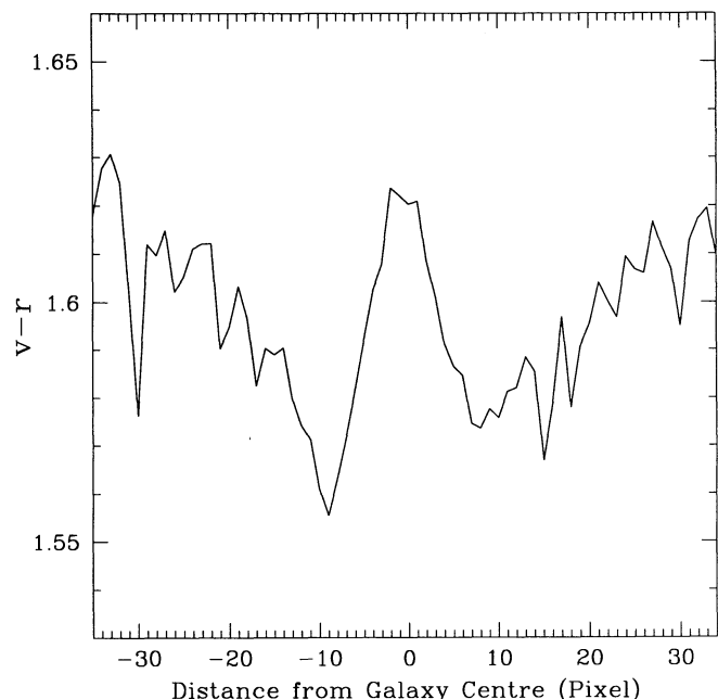
FIG. 4.—A cut across the dust lane, averaged over 10 rows around the galaxy center. The instrumental color v - r is shown.
