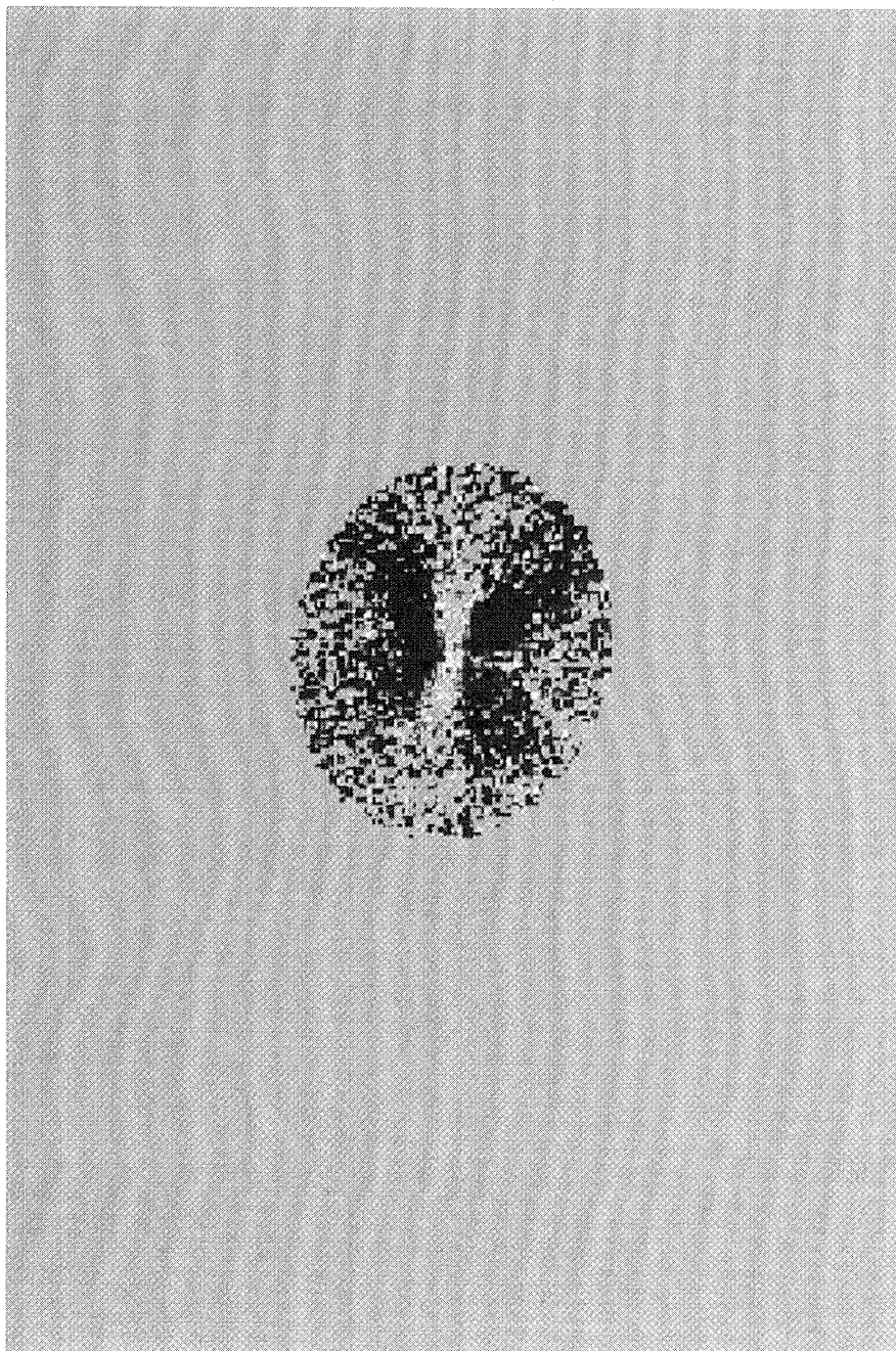
FIG. 3.— V - R_{\text{smooth}} image of NGC 4261 in false color. Each pixel is 0''.56 .
