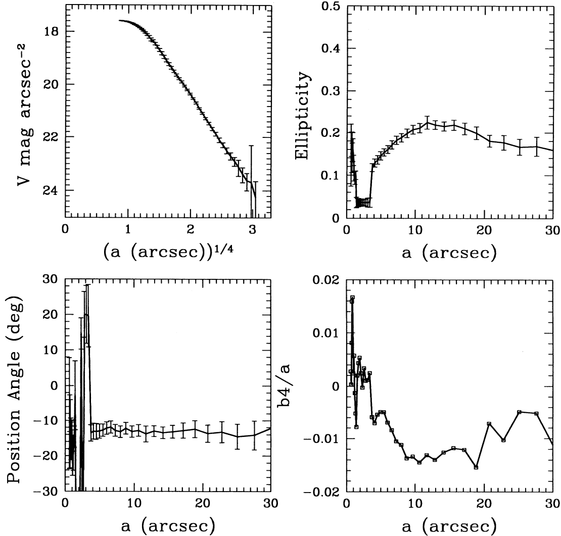
FIG. 1.—Semimajor axis profiles in the V band of surface brightness, ellipticity, position angle, and the boxiness coefficient b_4/a . The surface brightness is shown as a function of a^{1/4} , where a is the semimajor axis length of the isophotes.
