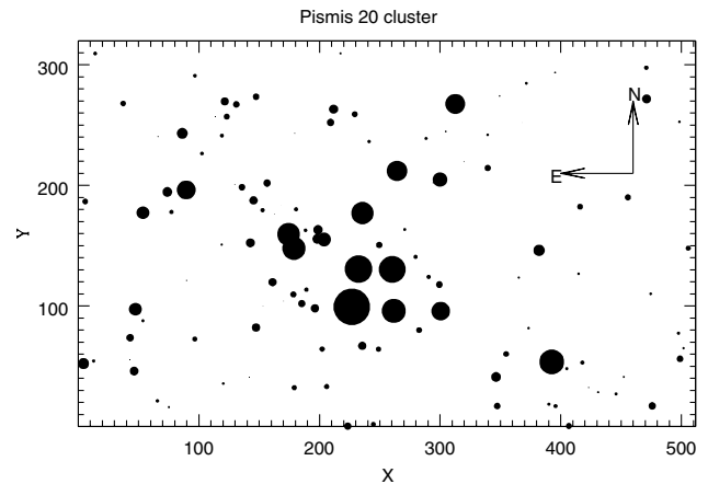
Figure 6. Identification map for the imaged region of the cluster Pismis 20. Other details are the same as in Fig. 1.
