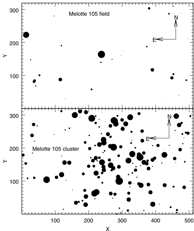
Figure 3. Identification maps for the imaged cluster and field regions of Melotte 105. Other details are the same as in Fig. 1.
