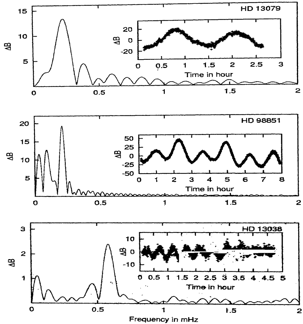
Figure 2. Lightcurve and FT of the other three variables discovered in the Naini Tal-Cape survey
