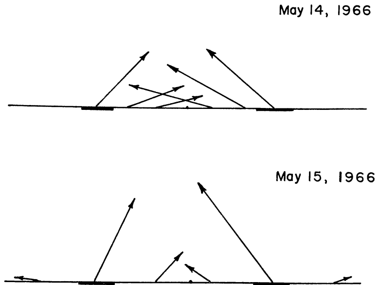
Fig. 4. Schematic pictures of the total field vector of a magnetic field at the sunspot group axis.
