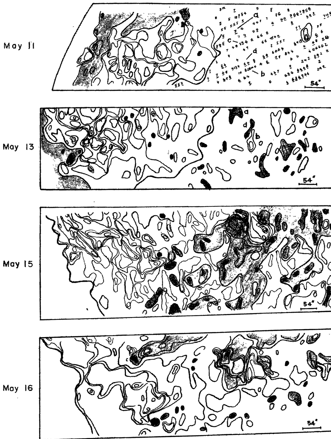
Fig. 2. Charts of the longitudinal magnetic-field component. Isogausses correspond to the field strengths 5, 15, 20, 50 gauss and > 50 gauss, respectively. Shaded areas are N polarity. A bold full line is the zero line of the field H_{\parallel} = 0 .
