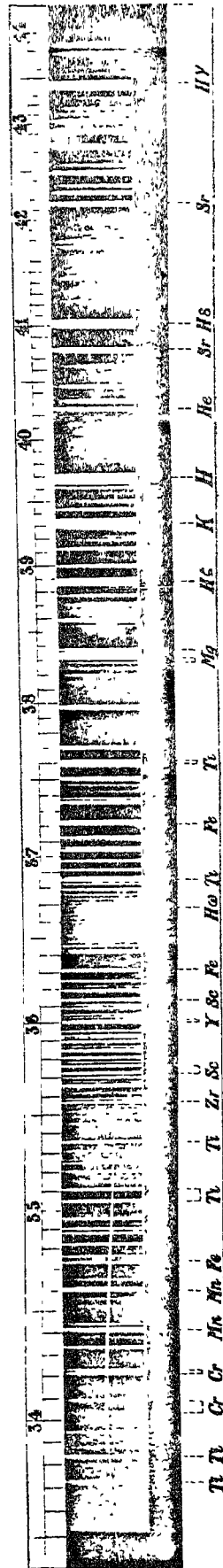
Spectrum of Lower Chromosphere—ultra-violet region. From photograph taken with a 2-inch prismatic camera at the Solar Eclipse of January 22nd, 1898.
