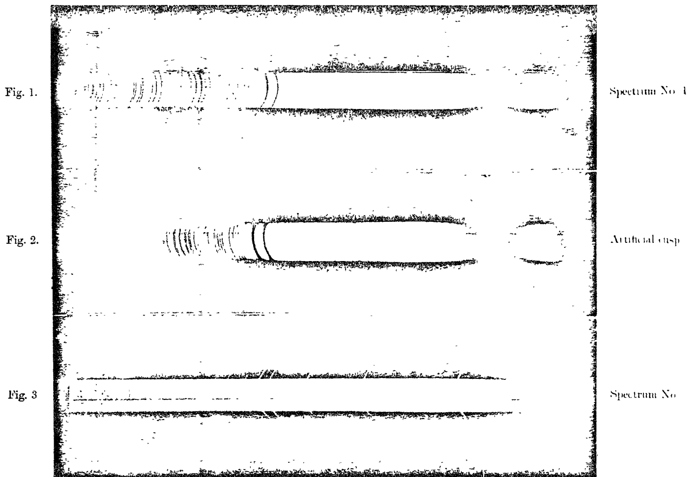
Comparison between cusp spectra photographed during the solar eclipse, and artificial cusp photographed in ordinary daylight—to show the relative faintness of the Fraunhofer lines in the eclipse spectra, and the great extension of the latter in the ultra-violet. (The absence of lines between F and H in each spectrum is due to over-exposure.)
