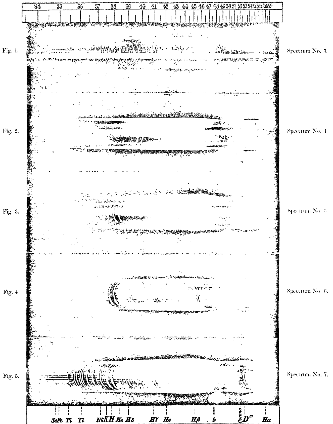
Spectra photographed during total phase. Eclipse of January 22nd, 1898.
