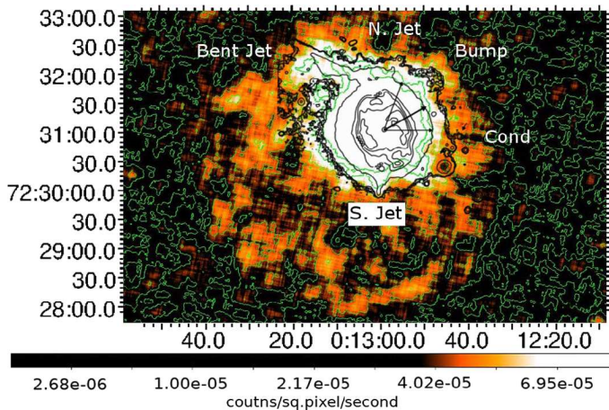
Fig. 5. Sketch of contoured H\alpha halo image illustrating interaction with ISM from Martin et al. (2002; dark contours) superposed on slightly smoothed FUV F169M image with green contours showing the FUV halo. We note the similarities between the images in the bent jet, the north jet (N. Jet), and the bump.
