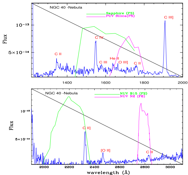
Fig. 1. IUE low-resolution nebular spectrum of NGC 40 (blue line) obtained at 6'' north and 13'' west of the central star. FUV and NUV are plotted at the top and bottom, respectively, with UVIT-filter effective areas (relative) shown. In the top panel , green denotes F169M FUV Sapphire and magenta denotes F172M FUV Silica, and in the bottom panel , green is N219M NUV B15 and magenta is N279N NUV N2.
