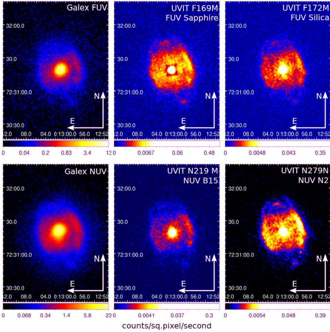
Fig. 2. Comparison of Galax images of NGC 40 with UVIT images. We note that the UVIT images provide better resolution and show structure in the nebula. The core of NGC 40 in F169M FUV Sapphire (top middle) is compared with N219M NUV B15 that shows mainly C II 2326 Å emission. C II image is very similar to low-excitation nebular line emissions seen in [S II] or [N II] (Meaburn et al. 1996) whereas F169M image shows several bright nebular condensations (also see Fig. 3). The axes are \alpha and \delta .
