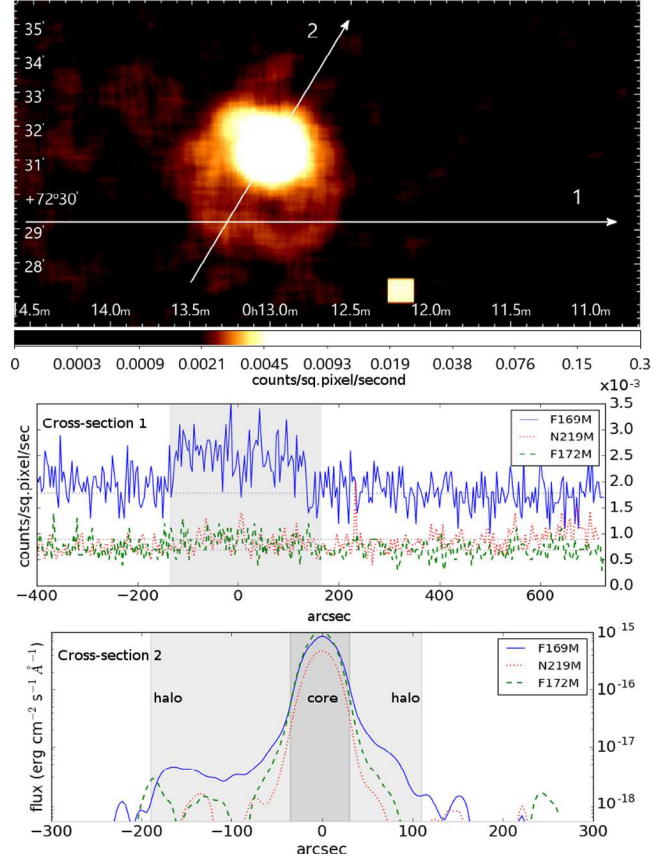
Fig. 4. Cross-cuts in the images of the nebula in three filters; F169M (blue), F172M (green), and N219M (red) made along the white lines shown in the slightly smoothed F169M image of the nebula (top). Cross-cuts of 8 pixel widths were obtained in all the images at the same locations (coordinates). The bottom cross-cut, which passes through the nebular core, is on a logarithmic scale and has been smoothed. We note the faint quasi-circular extended halo around the core of the nebula (on the south-east side). This region has been shown with a grey overlay in the plots. Despite having similar core fluxes in all three filters, only F169M shows the presence of the halo.
