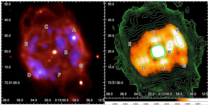
Fig. 3. X-ray image (left panel – blue emissions) superposed on H\alpha image is compared with the contoured F169M FUV Sapphire image (right panel). We note the similarities of the bright condensations of emission in both images and the overall elliptical shape.
