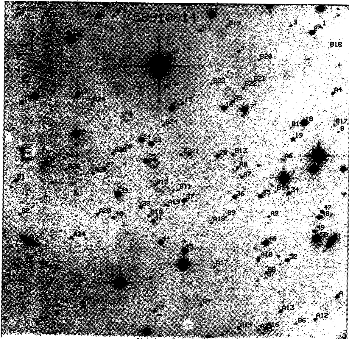
Fig 1. Field of GB910814 in I band with total exposure of 50m
