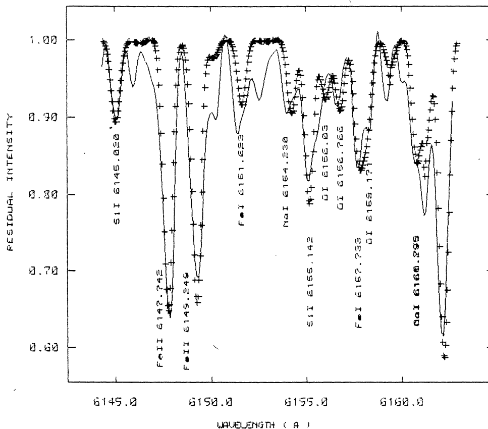
Figure 4. The agreement between the observed spectrum (continuous line) and synthesized spectra in the 6145–6162 Å region that contains O I lines.
