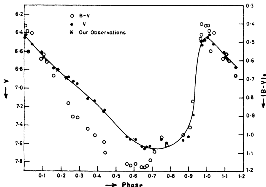
Figure 2. Light curve of RZ Vel using the observation of Mitchell et al. (1964). The phases at which our spectra were obtained are shown by * symbol.
