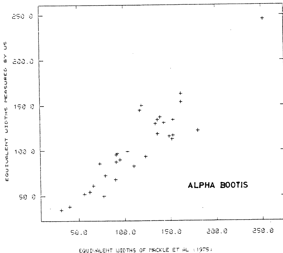
Figure 1. Equivalent widths measured by us are compared with those of Mäcke et al. (1975) for alpha Bootis.
