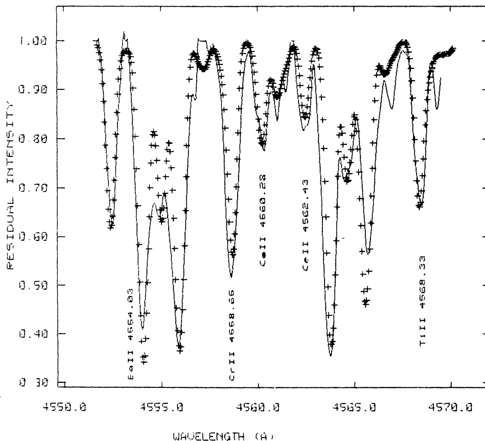
Figure 3. The agreement between the observed spectrum (continuous line) and synthesized spectra in the 4550–4570 Å region that includes Ba II and Ce II lines.
