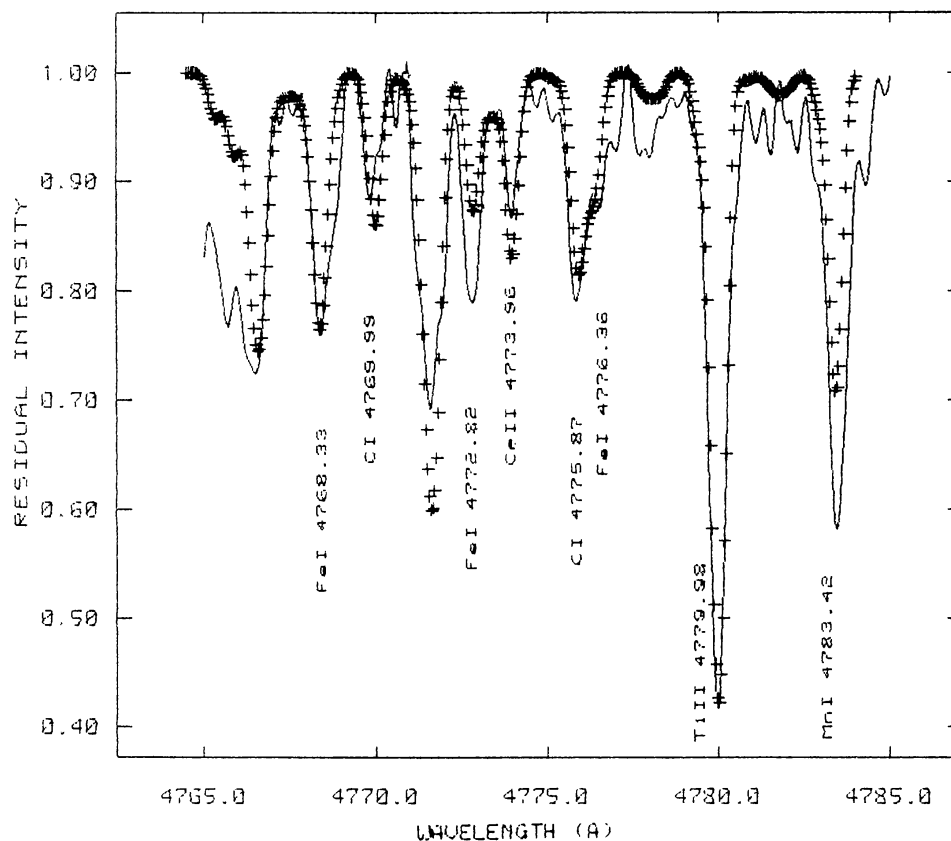
Figure 5. The agreement between the observed spectrum (continuous line) and synthesized spectra in the 4765–4785 Å region that contains C I lines.
