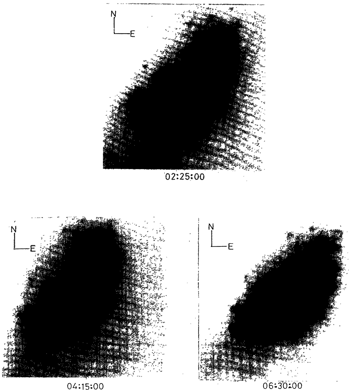
Fig. 1b. White-light photoheliograms on the flare day, June 11, 1991 at 02:25:00, 04:15:00, 06:30:00 UT.
