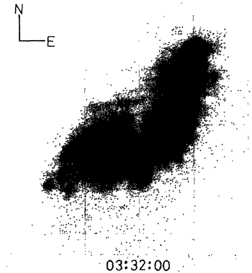
Fig. 1c. Post-flare white-light photoheliogram on June 12, 1991 at 03:32:00 UT.
